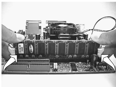
Step 4: Press the latches into the notches of the RAM module
