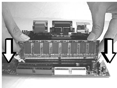
Step 3: Insert the RAM module into the DIMM Socket
