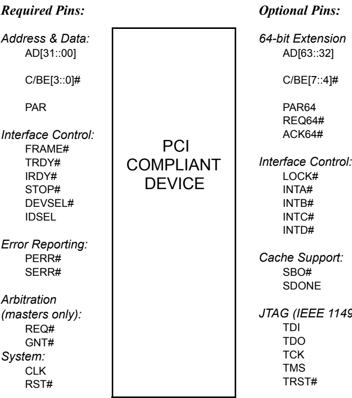
PCI Pin List
