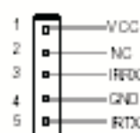
IrDA Connector
