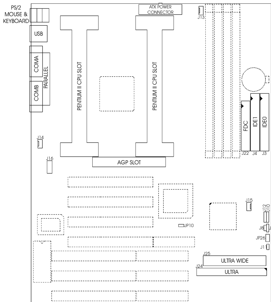
Fig 3 Connector Location
