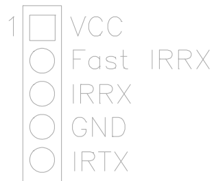
Fig. 9 IrDA Connector
