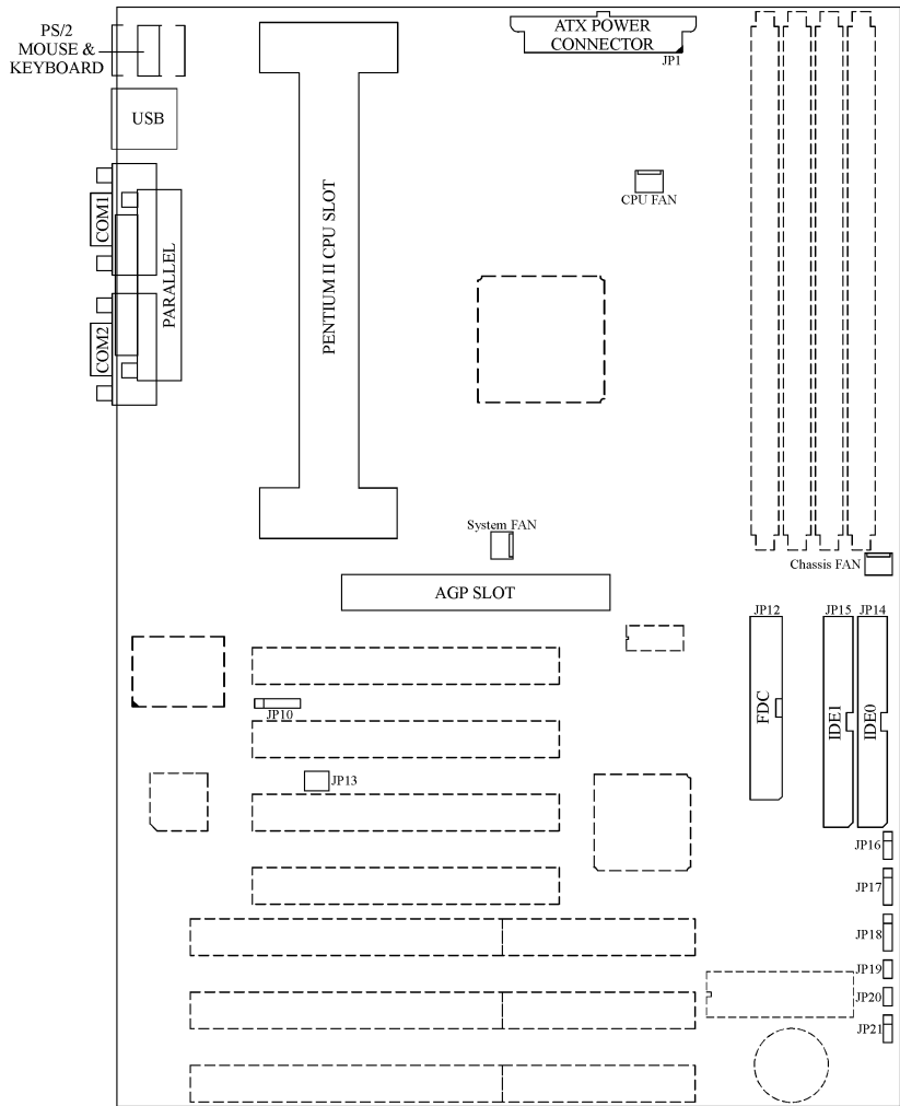
Fig 3 Connector Location
