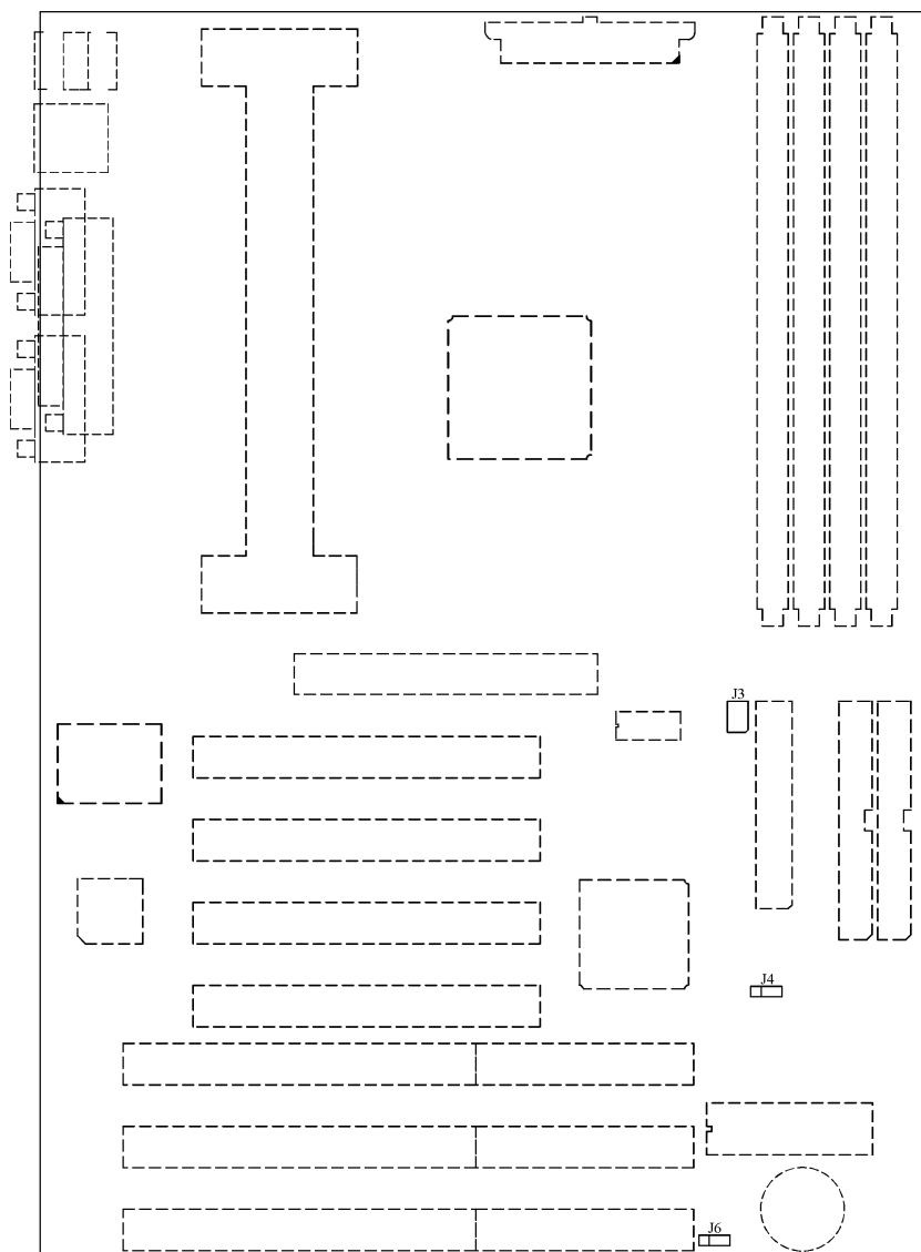
Fig. 2 Jumper Location of the mainboard
