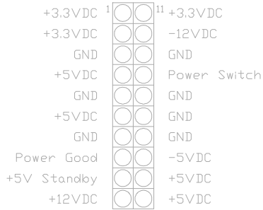
Fig. 4 ATX Power Supply Connector
