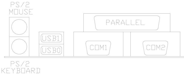
Fig. 12 I/O Connector
