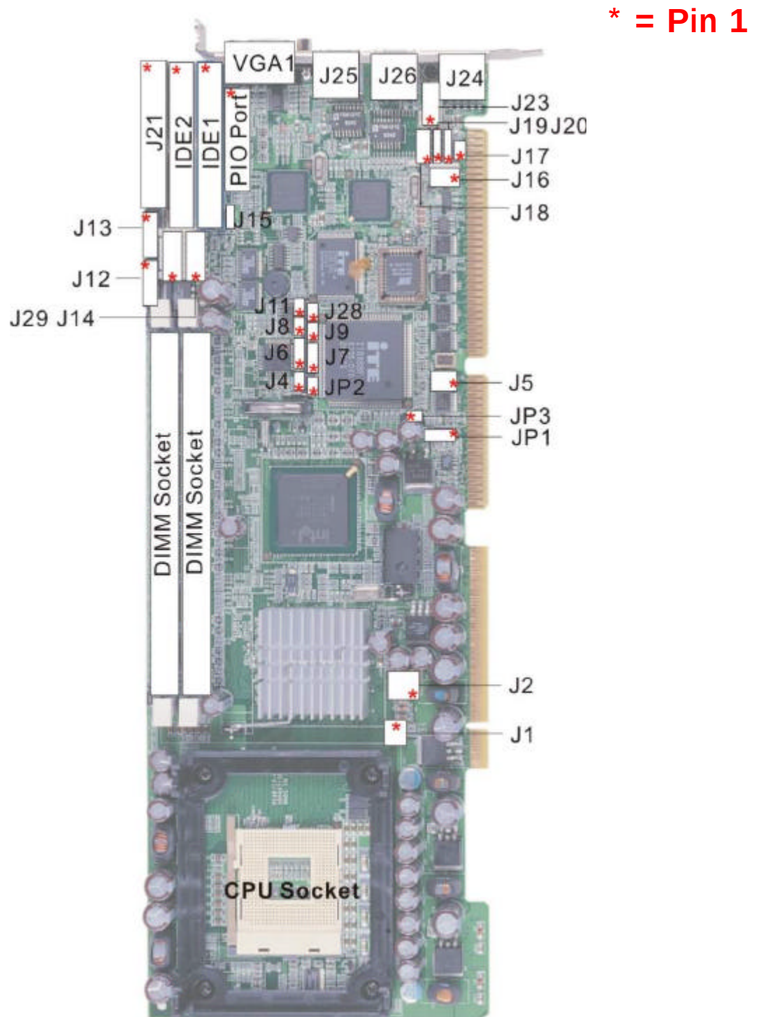
Figure 2-2 : Jumper Locations
