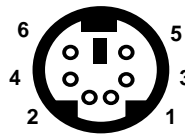
PS/2 Keyboard (6-pin Female)
