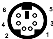
PS/2 Mouse (6-pin Female)
