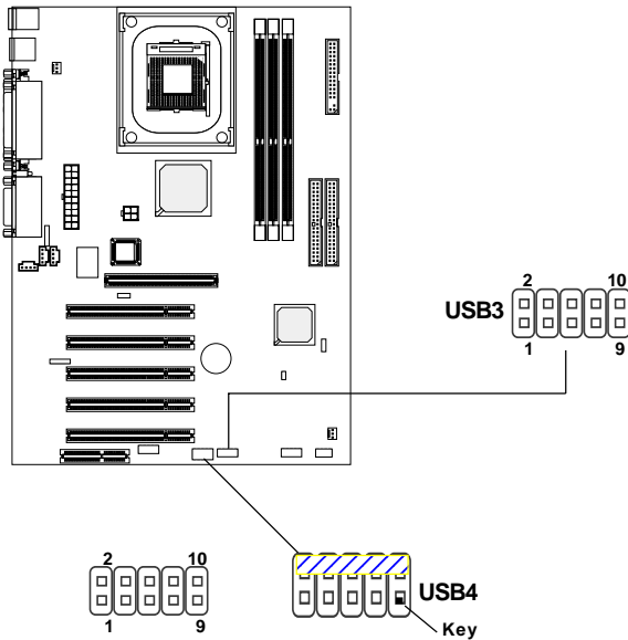
USB3 Pin Definition
