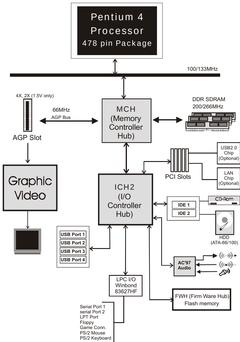
Figure 5: System Block Diagram
