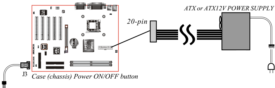
Figure 4: Simple ATX or ATX12V Power ON/OFF Controller
