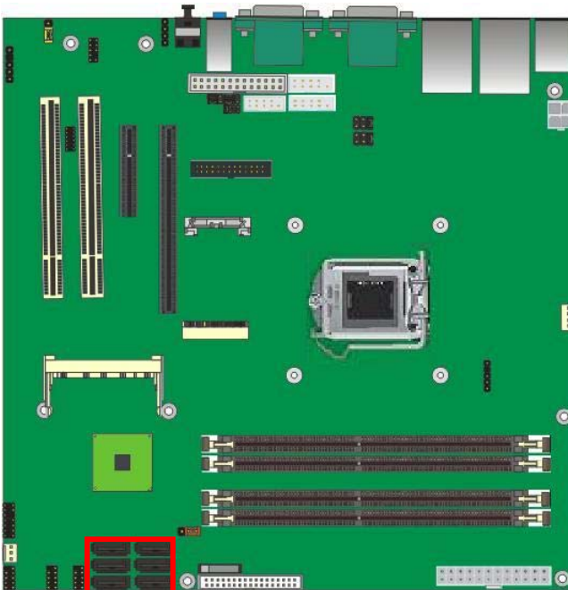
SATA1/2/3/4/5/6
