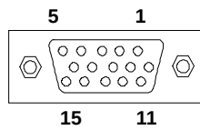
DB 15-Pin Female Connector
