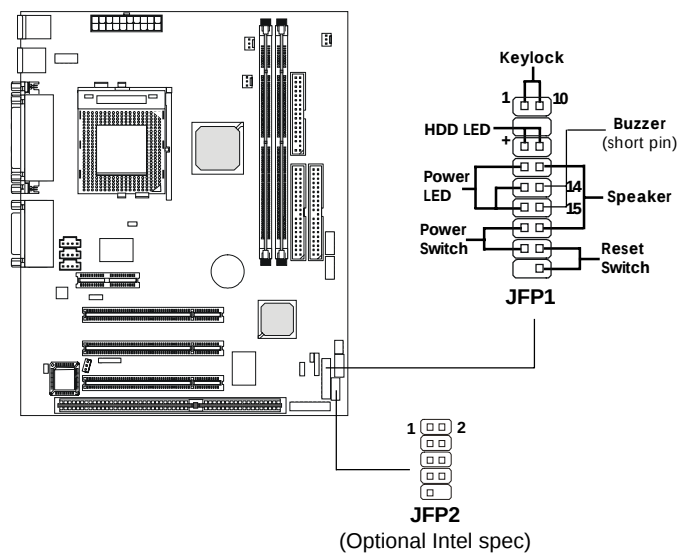
JFP2 Pin Definition
