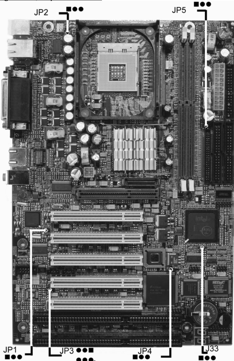
Figure 1-1 Jumper Locations
