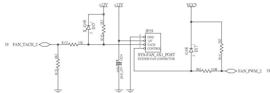
Chassis FAN for SYSTEM
