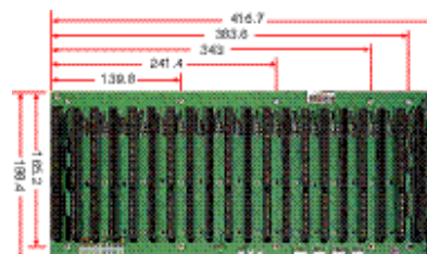
20-Slot ISA Passive Backplane
