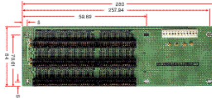
Horizontal 6-Slot ISA Passive Backplane
