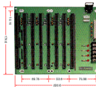
8-Slot ISA Passive Backplane
