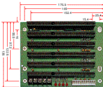
6-Slot ISA Passive Backplane
