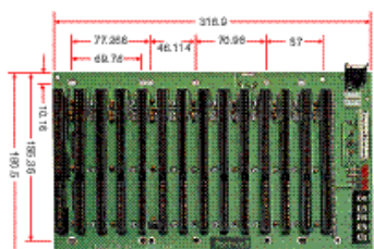
14-Slot ISA Passive Backplane
