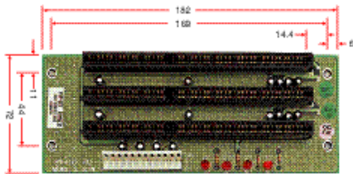
3-Slot ISA Passive Backplane
