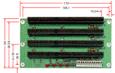
4-Slot ISA Passive Backplane
