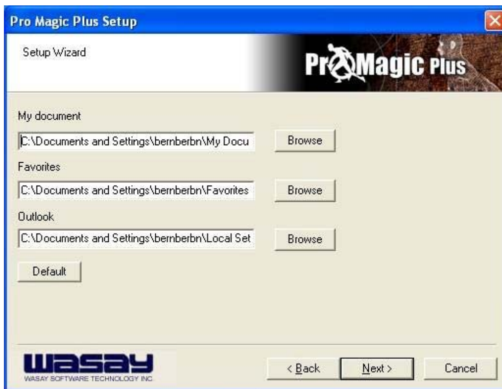
graph 4
