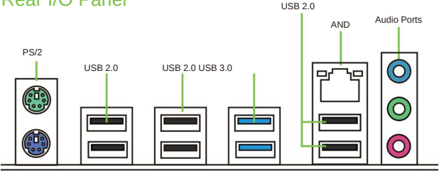
Figure 1-2 Overall rear I/O panel display
