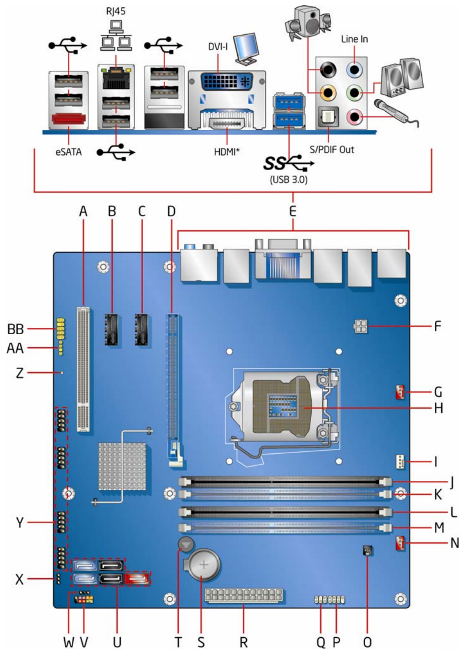
Figure 1. Intel Desktop Board DH67BL Components
