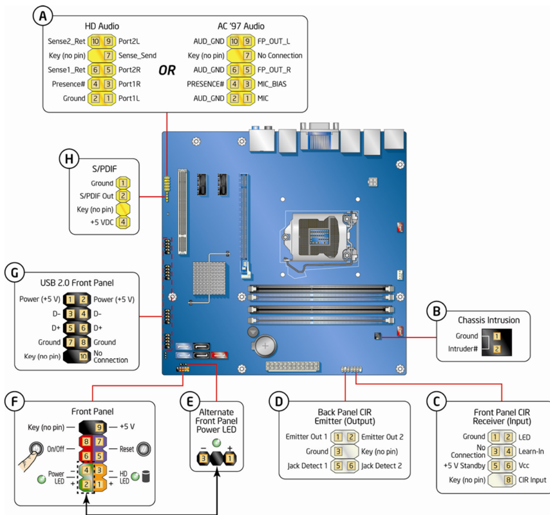
Figure 20. Internal Headers
