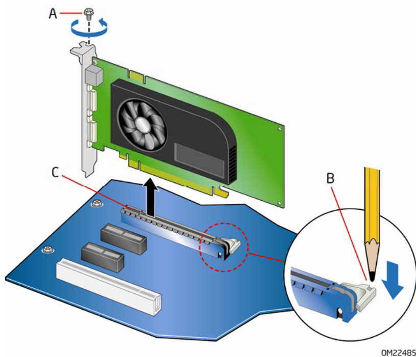
Figure 18. Removing a PCI Express x16 Graphics Card
