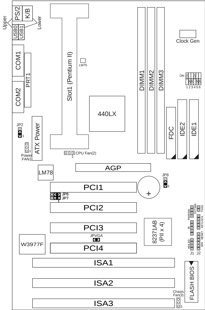
Figure 1–1. Motherboard Layout
