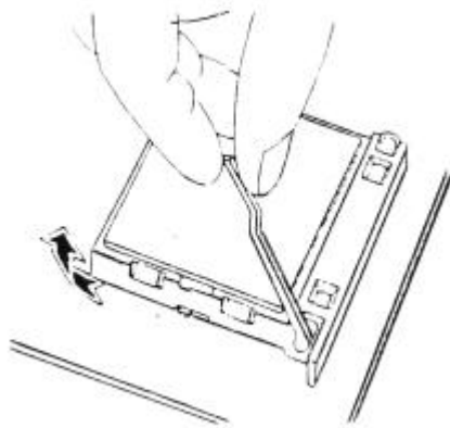
Figure 3-3 Installing CPU
