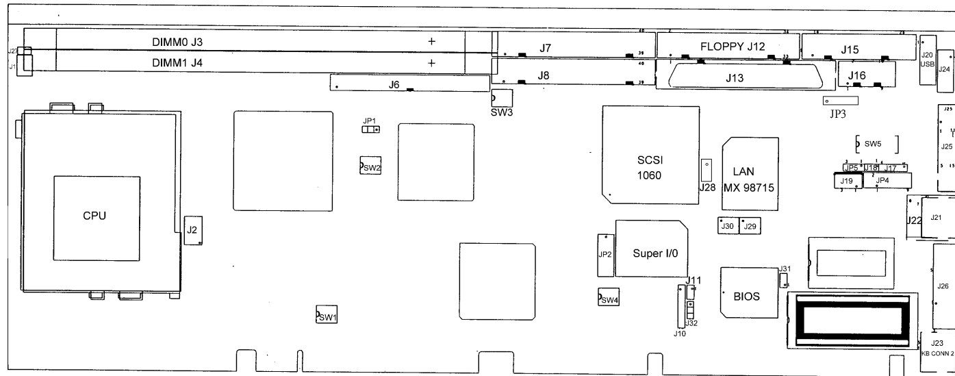
Figure 2-2 Switches and Connectors position – Version E and afterwards
