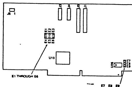
FIGURE 7-1 WD1003-WA2 JUMPER LOCATIONS
