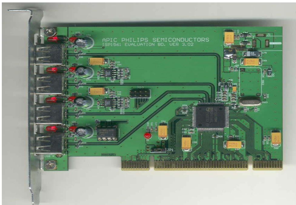
Figure I-1: ISP1561 Evaluation Board
