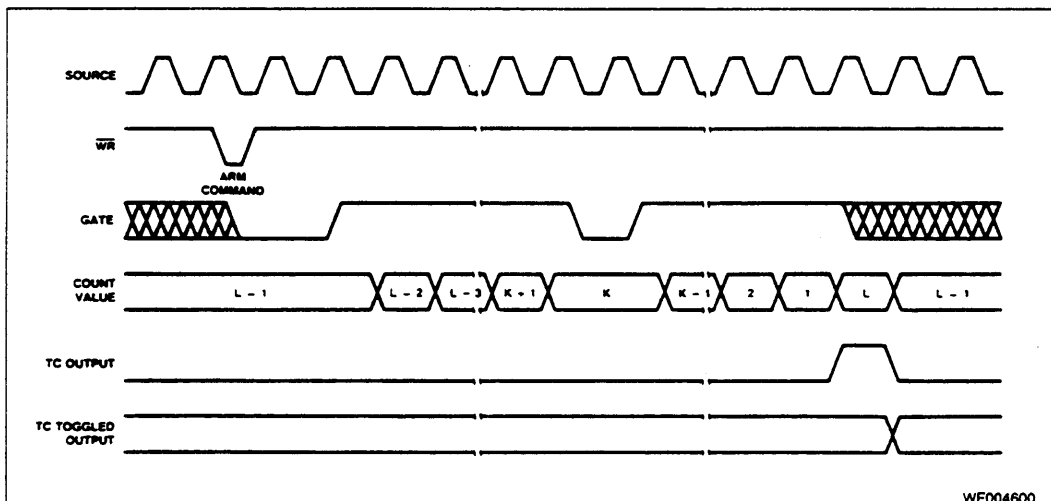
Figure 15b. Mode B Waveforms
