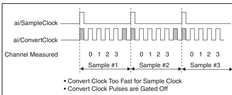
Figure 4-19. ai/ConvertClock Too Fast
