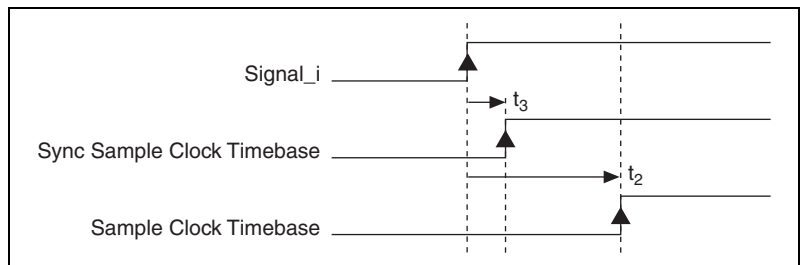
Figure B-24. External Update Source Clock Insertions Timing Diagram
