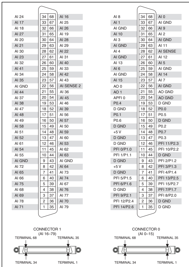
Figure A-43. USB-6255 Mass Termination Pinout
