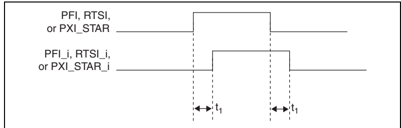
Figure B-42. Pin to Internal Signal Delays Timing Diagram
