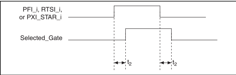
Figure B-43. Selected Gate Delays Timing Diagram
