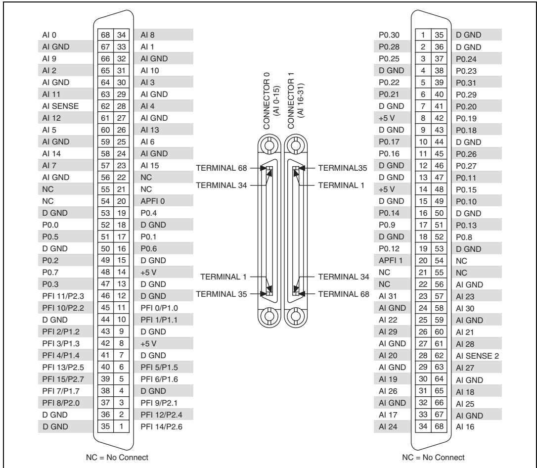
Figure A-40. PCI/PXI-6254 Pinout
