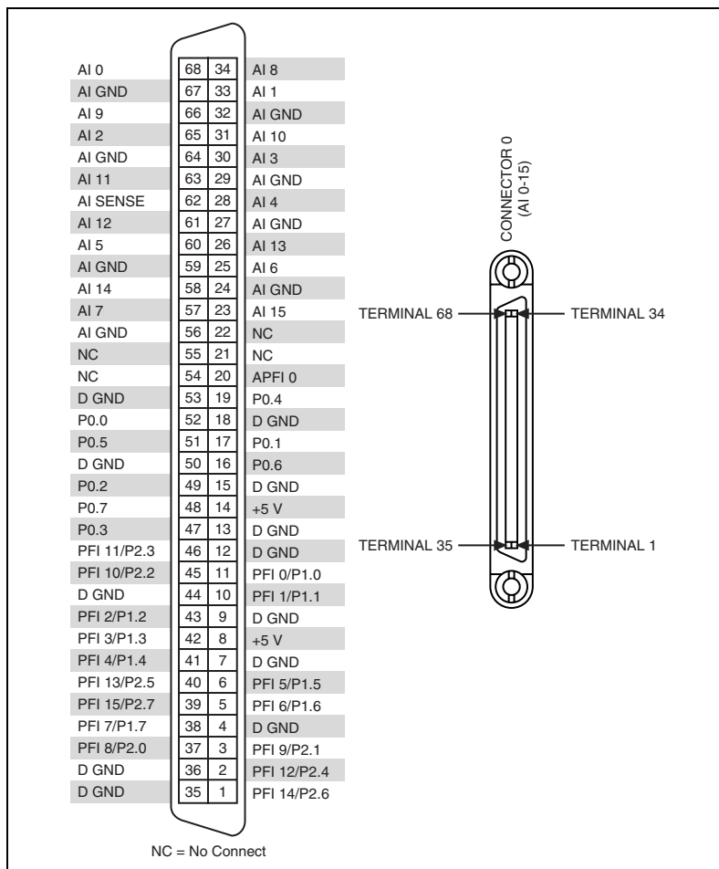
Figure A-56. PCI/PXI-6280 Pinout
