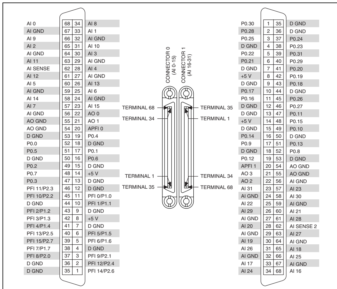
Figure A-44. NI PCI/PCIe/PXI/PXle-6259 Pinout
