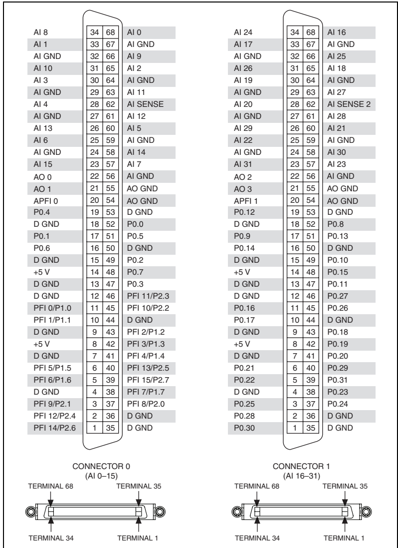
Figure A-55. USB-6259 Mass Termination Pinout
