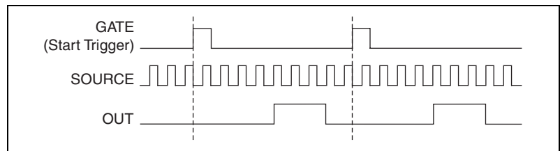
Figure 7-23. Retriggerable Single Pulse Generation
