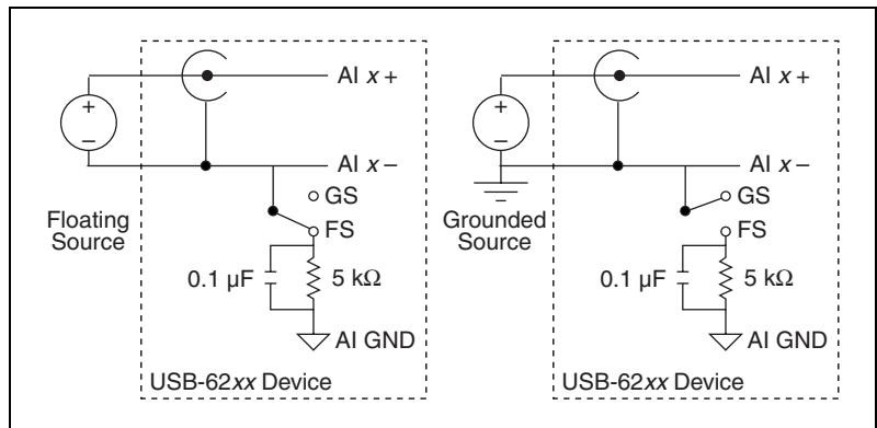
Figure A-21. Analog Input Circuitry
