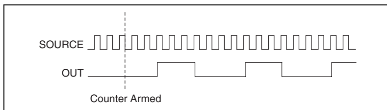
Figure 7-24. Continuous Pulse Train Generation
