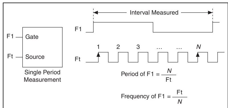
Figure 7-10. Method 1
