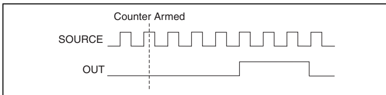
Figure 7-21. Single Pulse Generation
