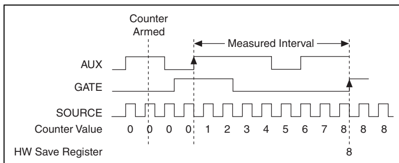
Figure 7-19. Single Two-Signal Edge-Separation Measurement
