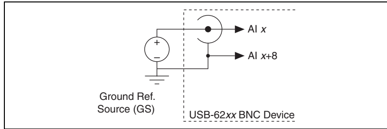
Figure A-22. Single-Ended Channels
