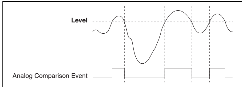
Figure 11-4. Above-Level Analog Triggering Mode
