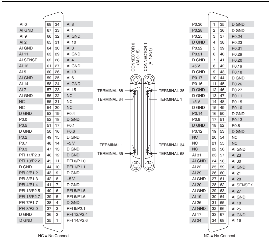
Figure A-13. PCI/PXI-6224 Pinout
