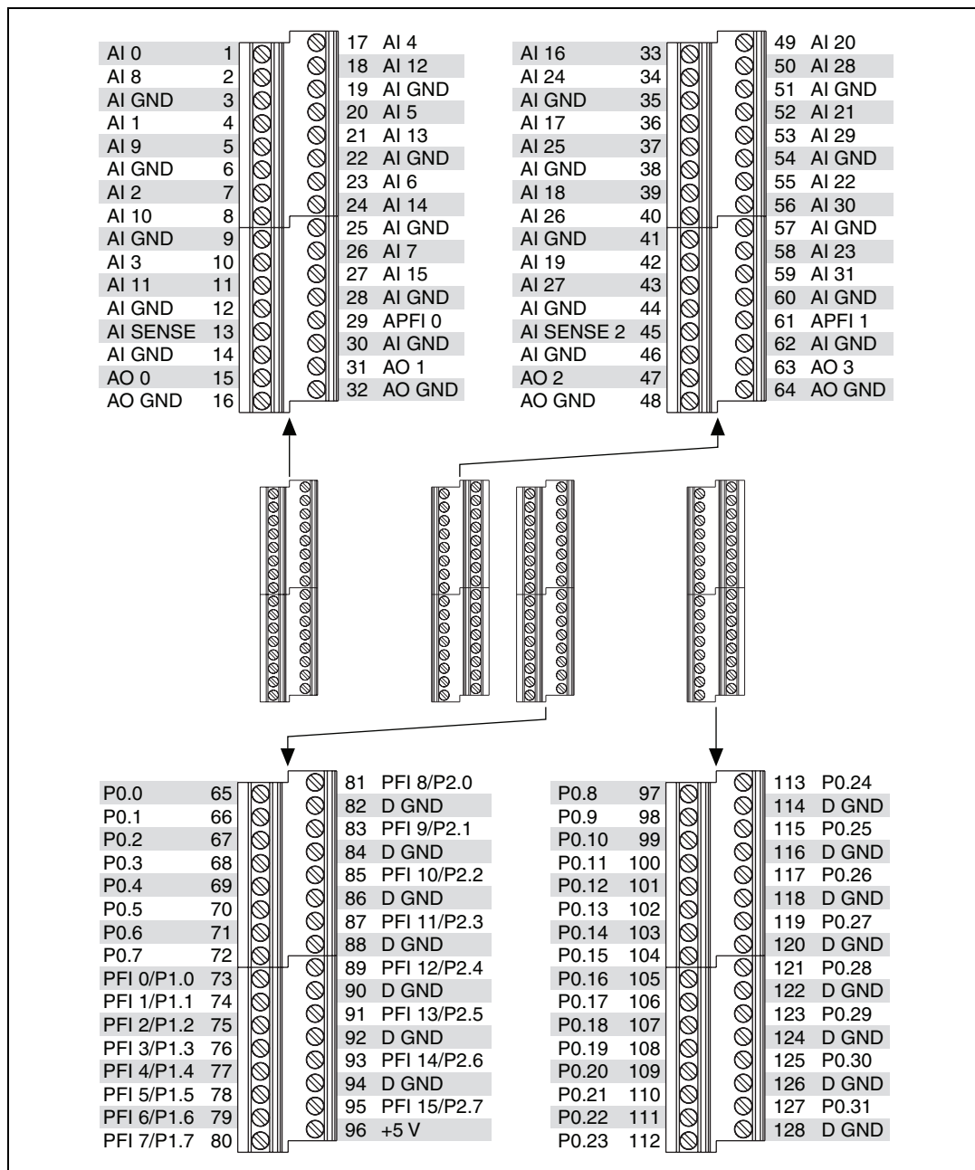
Figure A-45. USB-6259 Screw Terminal Pinout
