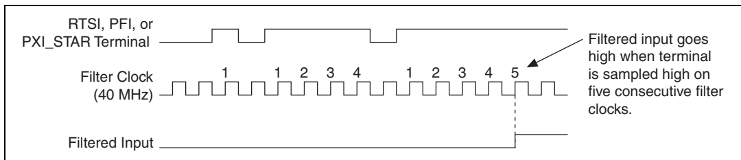
Figure 9-3. Filter Example
