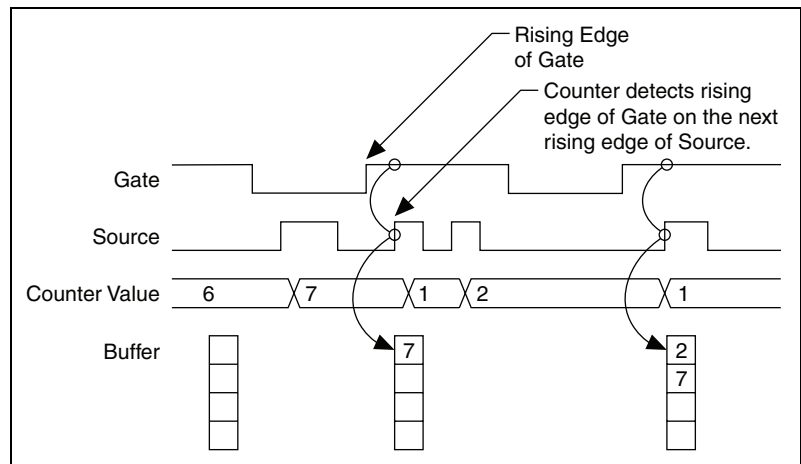
Figure 7-30. Duplicate Count Prevention Example
