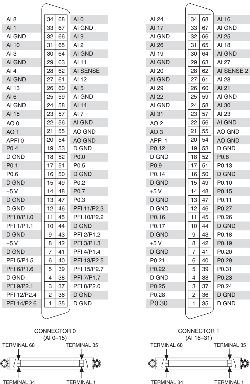
Figure A-63. USB-6289 Mass Termination Pinout
