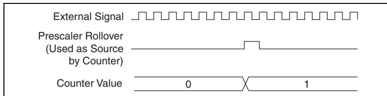
Figure 7-29. Prescaling
