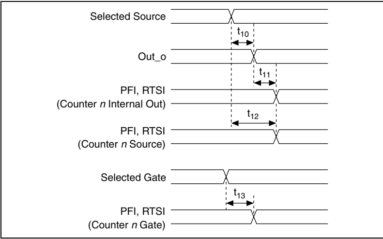
Figure B-50. Output Delays
