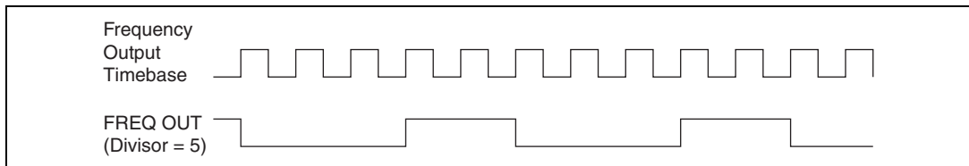
Figure 7-26. Frequency Generator Output Waveform
