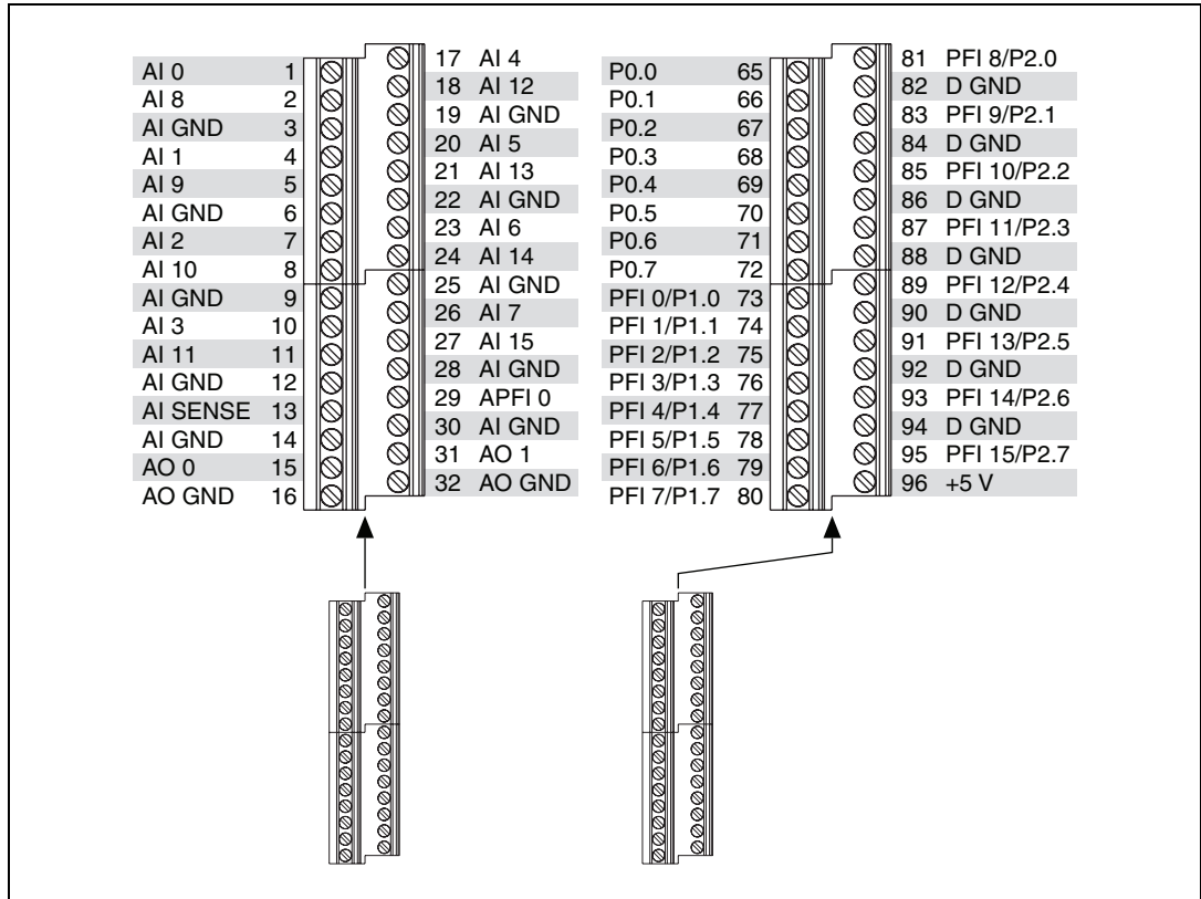
Figure A-29. USB-6251 Screw Terminal Pinout
