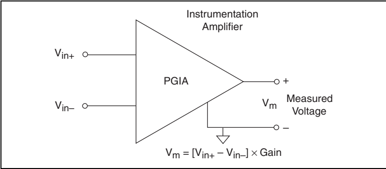
Figure 4-2. NI-PGIA
