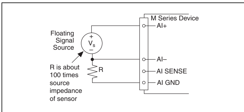
Figure 4-5. Differential Connections for Floating Signal Sources with Single Bias Resistor
