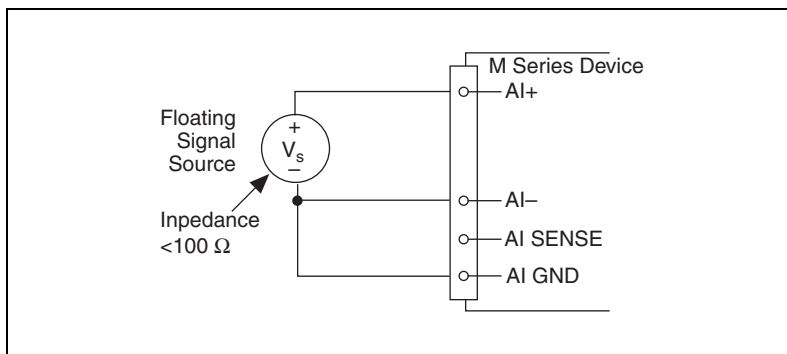
Figure 4-4. Differential Connections for Floating Signal Sources without Bias Resistors
