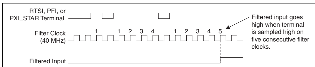
Figure 7-28. Filter Example
