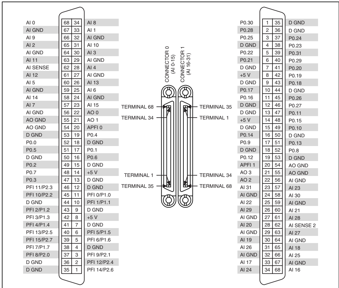
Figure A-61. PCI/PXI-6289 Pinout
