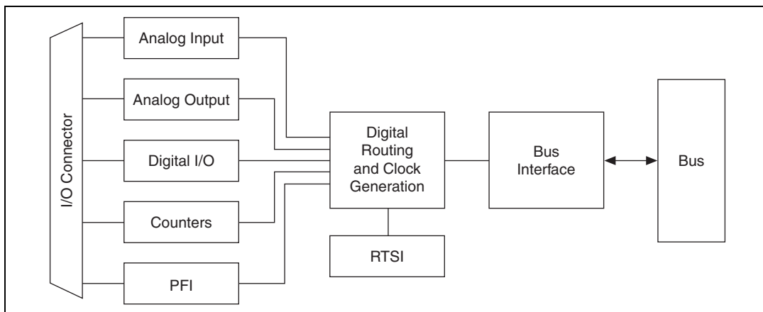
Figure 2-2. General M Series Block Diagram
