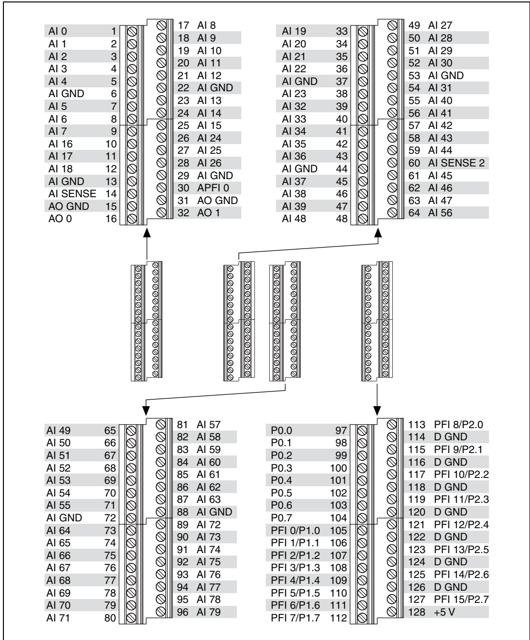
Figure A-42. USB-6255 Screw Terminal Pinout
