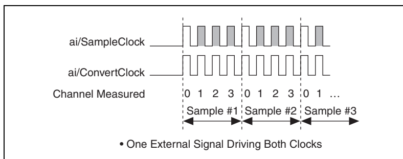
Figure 4-22. Single External Signal Driving ai/SampleClock and ai/ConvertClock Simultaneously
