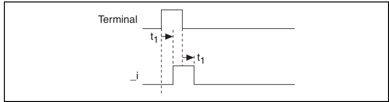
Figure B-23. Input Timing Diagram
