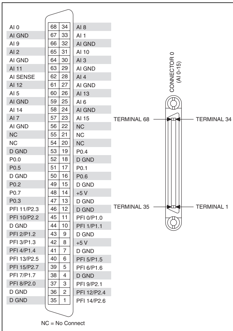
Figure A-1. PCI/PXI-6220 Pinout
