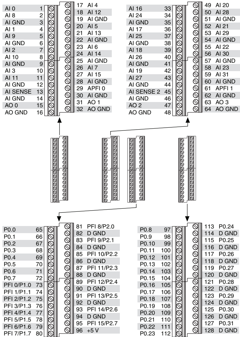
Figure A-62. USB-6289 Screw Terminal Pinout
