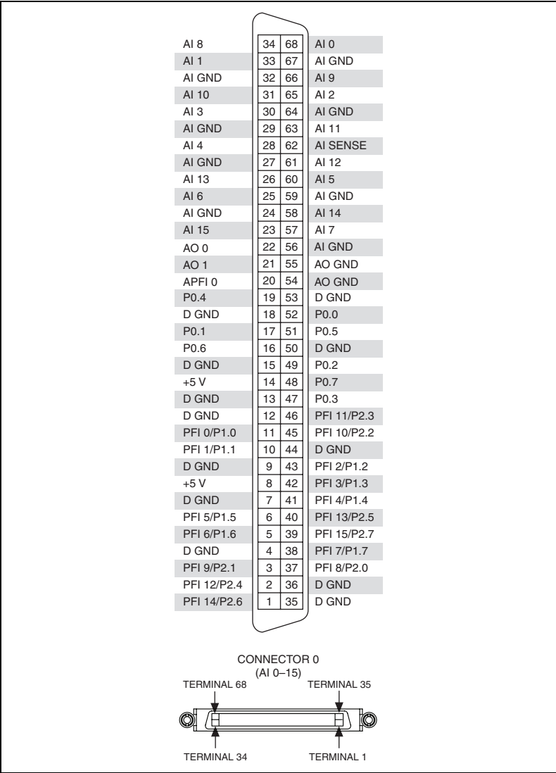
Figure A-39. USB-6251 Mass Termination Pinout
