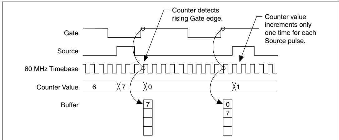
Figure 7-32. Duplicate Count Prevention Example
