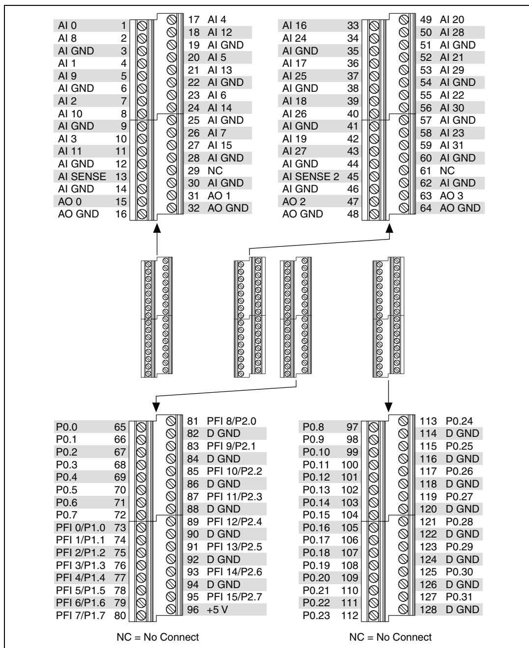
Figure A-18. USB-6229 Screw Terminal Pinout
