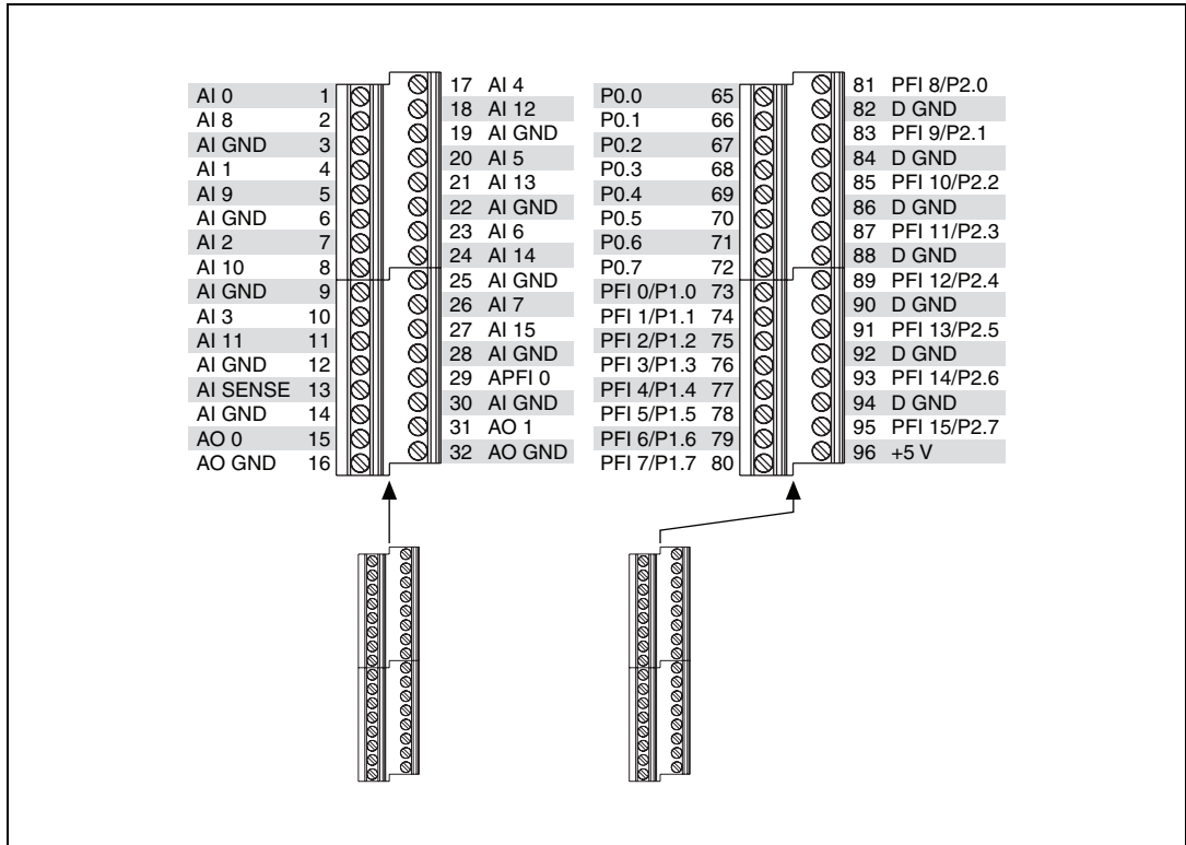
Figure A-58. USB-6281 Screw Terminal Pinout
