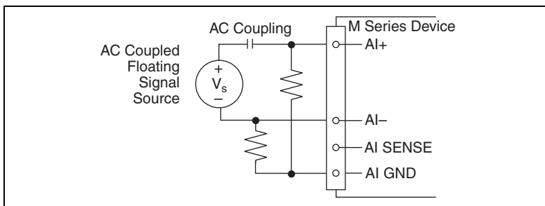
Figure 4-7. Differential Connections for AC Coupled Floating Sources with Balanced Bias Resistors
