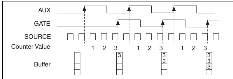
Figure 7-20. Buffered Two-Signal Edge-Separation Measurement
