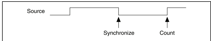
Figure 7-34. Other Internal Source Mode
