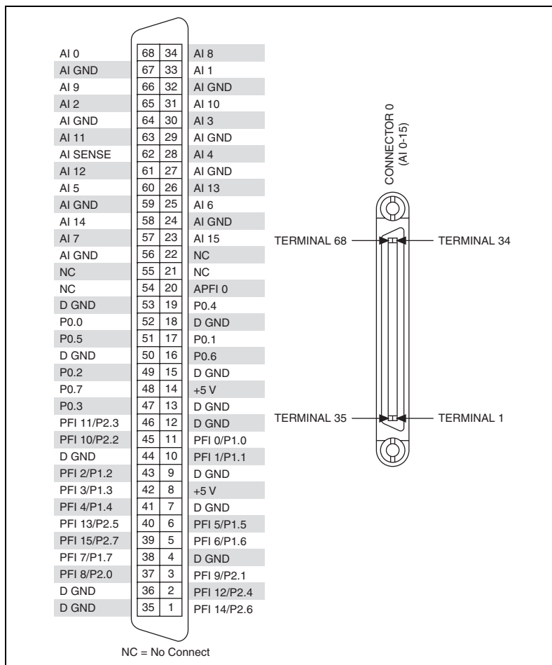
Figure A-27. PCI/PXI-6250 Pinout
