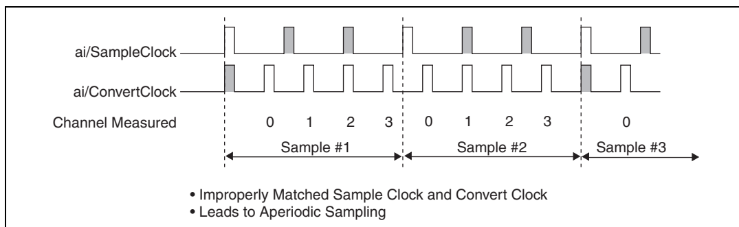
Figure 4-20. ai/SampleClock and ai/ConvertClock Improperly Matched
