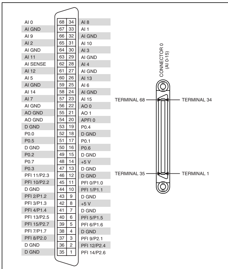
Figure A-57. PCI/PXI-6281 Pinout
