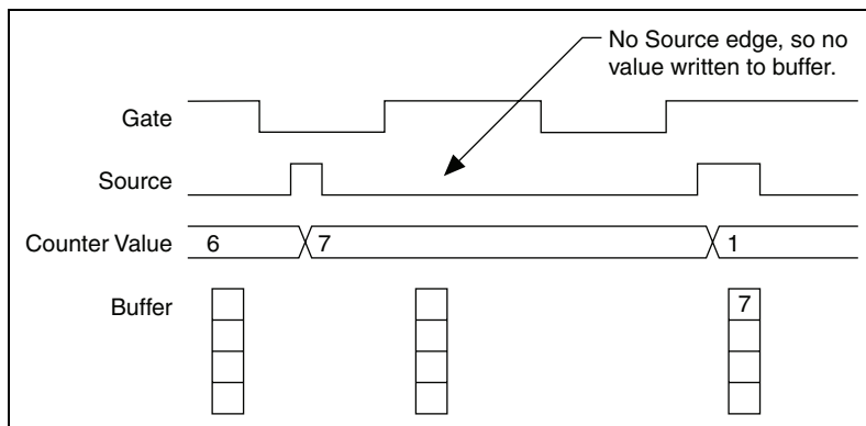
Figure 7-31. Duplicate Count Example
