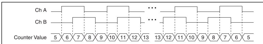
Figure 7-16. X4 Encoding
