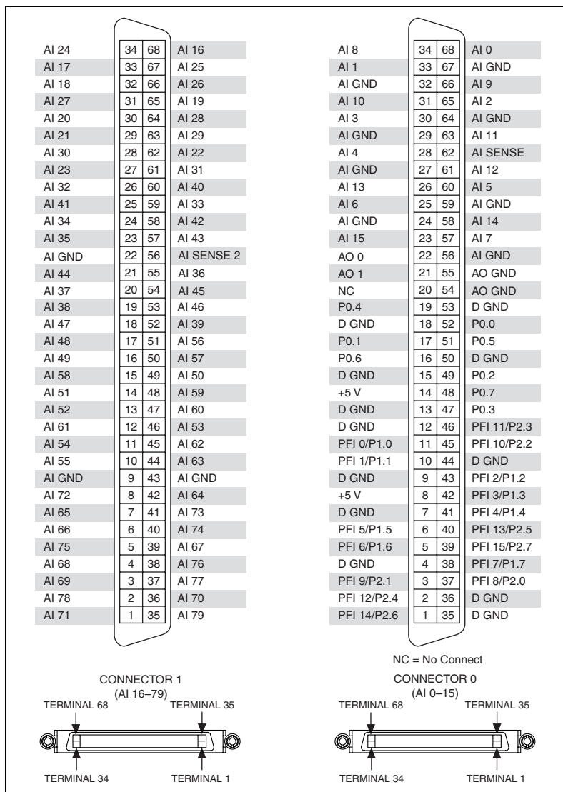
Figure A-16. USB-6225 Mass Termination Pinout
