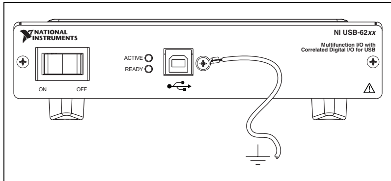
Figure 3-1. Grounding a USB-62xx Device through the Ground Lug Screw
