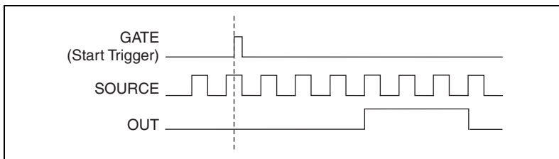
Figure 7-22. Single Pulse Generation with Start Trigger
