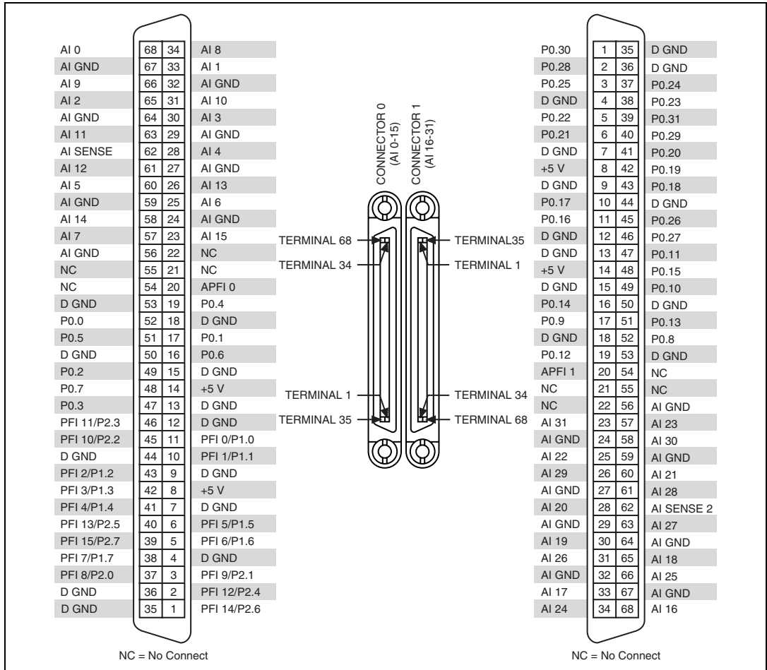
Figure A-60. PCI/PXI-6284 Pinout
