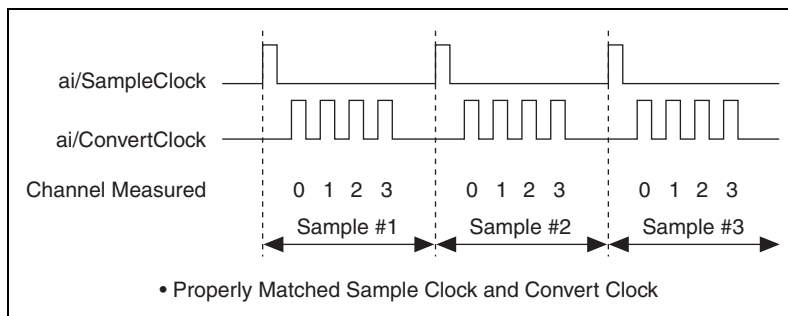
Figure 4-21. ai/SampleClock and ai/ConvertClock Properly Matched
