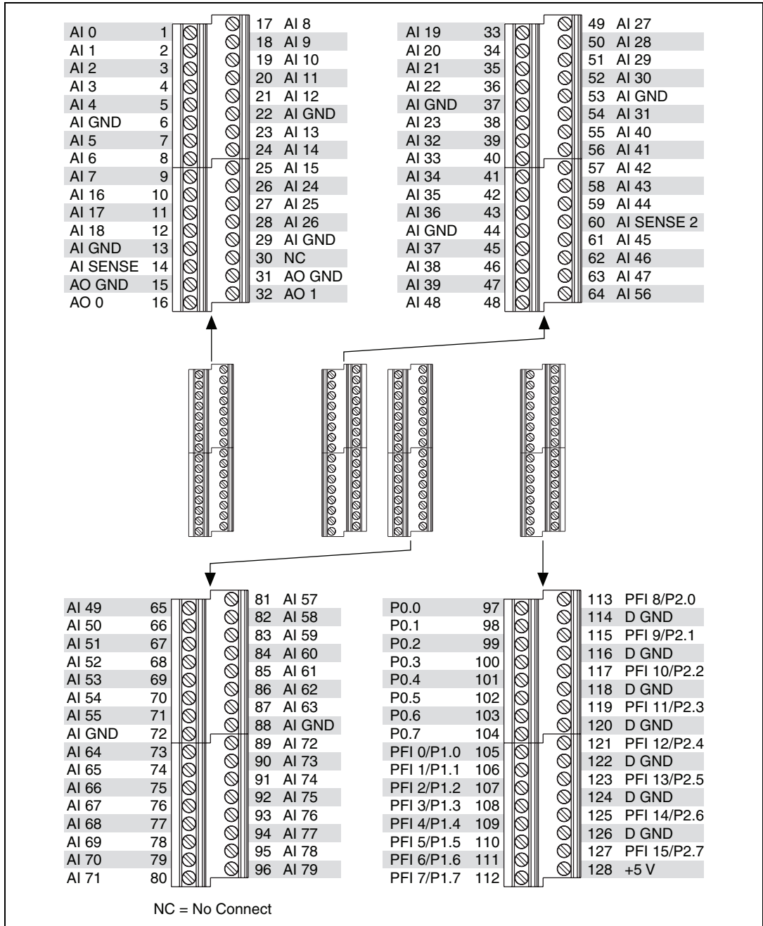
Figure A-15. USB-6225 Screw Terminal Pinout
