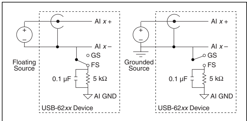
Figure A-48. Analog Input Circuitry
