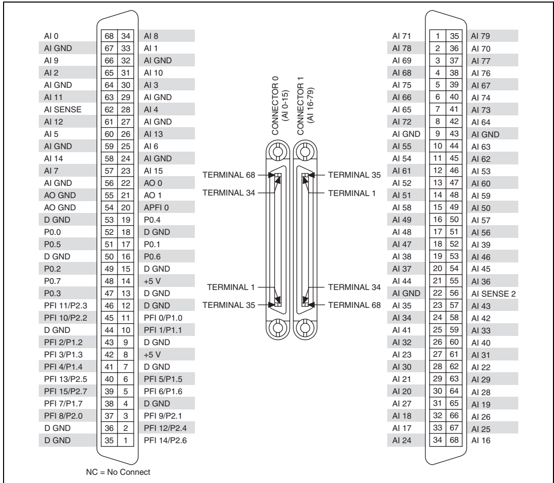
Figure A-41. PCI/PXI-6255 Pinout
