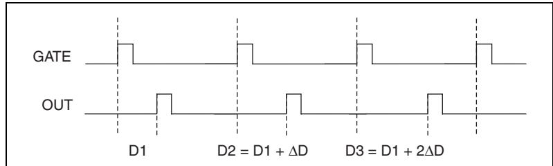
Figure 7-27. Pulse Generation for ETS
