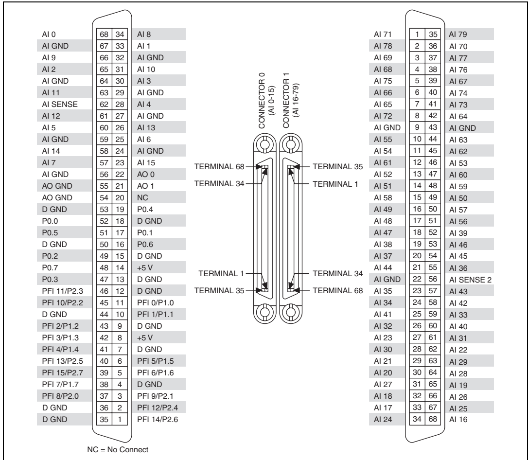
Figure A-14. PCI/PXI-6225 Pinout
