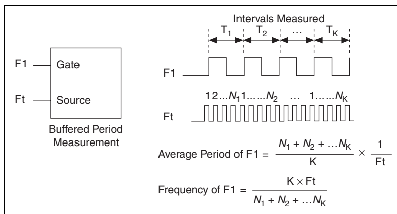
Figure 7-11. Method 1b
