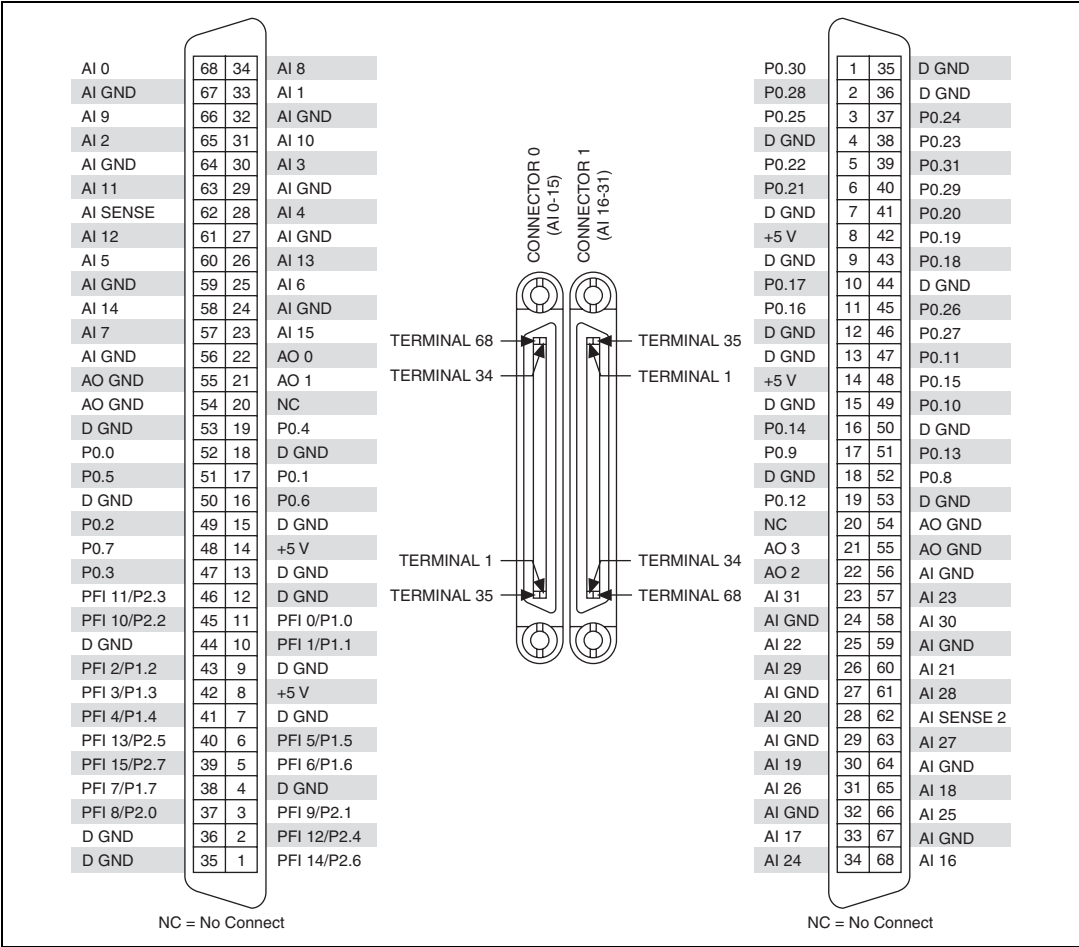
Figure A-17. PCI/PXI-6229 Pinout
