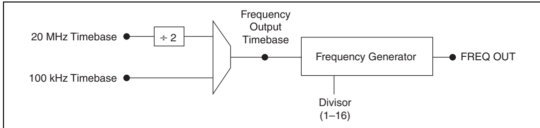
Figure 7-25. Frequency Generator Block Diagram
