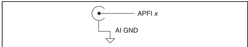
Figure A-52. Analog Programmable Function Interface Circuitry
