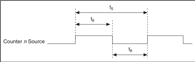
Figure B-46. Counter n Source Timing Requirements
