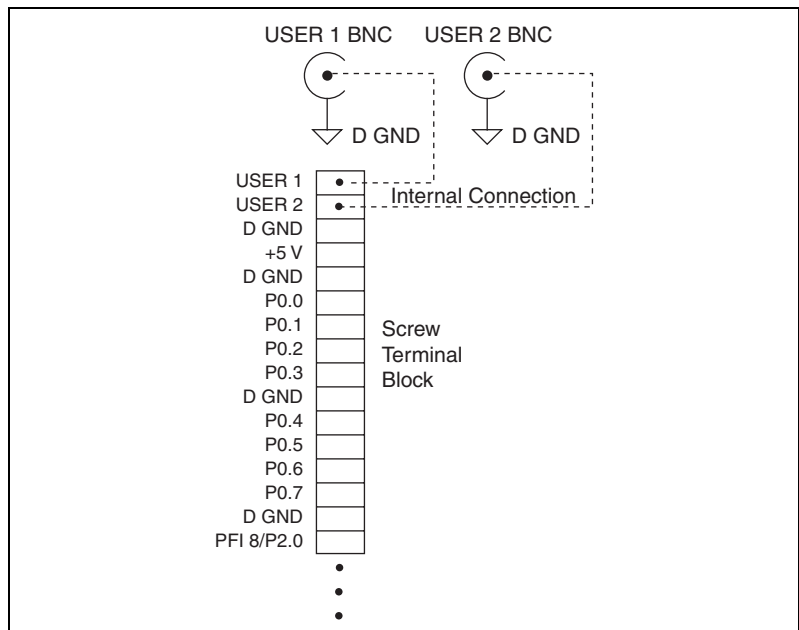
Figure A-25. USER 1 and USER 2 BNC Connections
