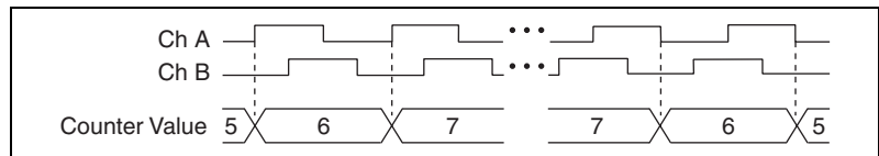
Figure 7-14. X1 Encoding
