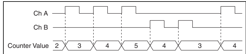
Figure 7-18. Measurements Using Two Pulse Encoders
