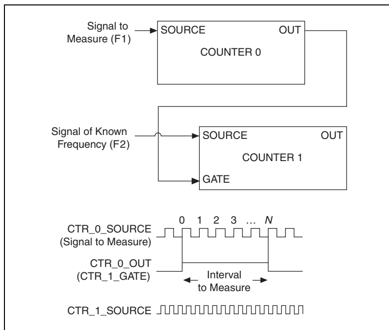
Figure 7-13. Method 3
