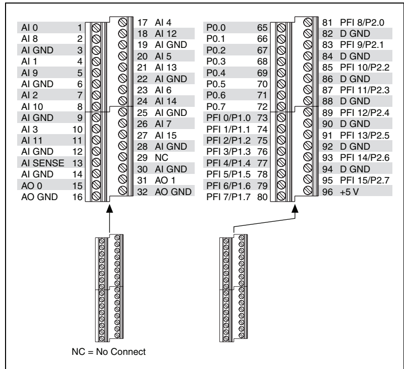
Figure A-4. USB-6221 Screw Terminal Pinout
