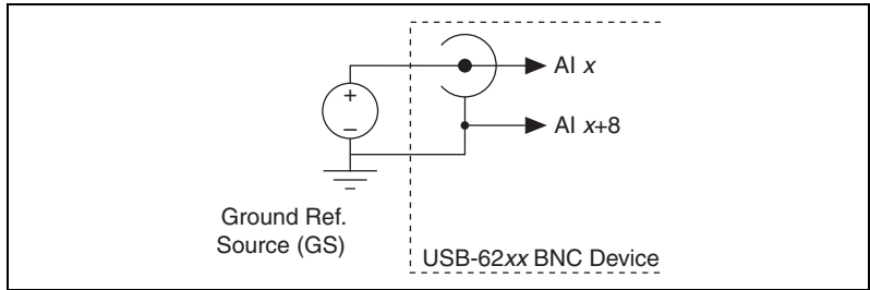
Figure A-33. Single-Ended Channels
