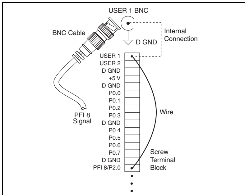
Figure A-26. Connecting PFI 8 to USER 1 BNC
