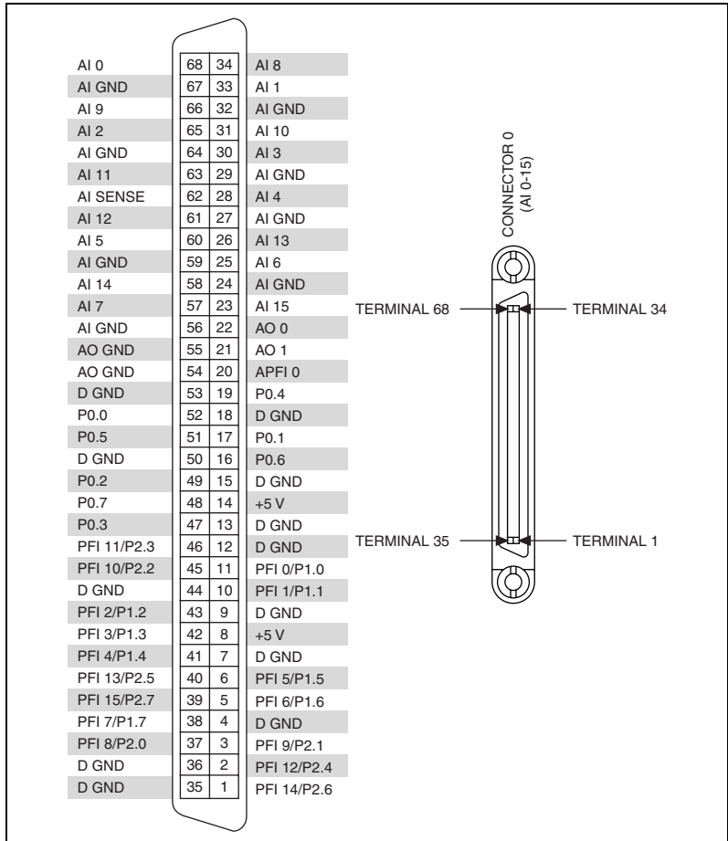
Figure A-28. NI PCI/PCIe/PXI/PXIe-6251 Pinout
