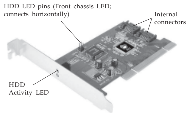
Figure 1. SATA II-150 PCI Board Layout
