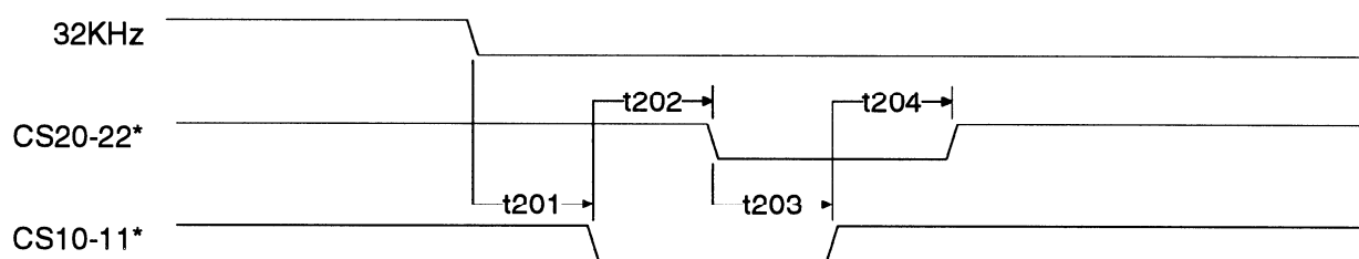
Figure 31. Timing for DRAM Suspend Mode Refresh
