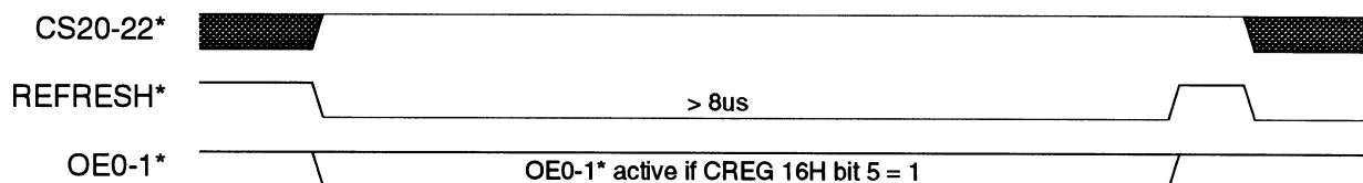
Figure 33. Functional Timing for PSRAM Suspend Mode Refresh
