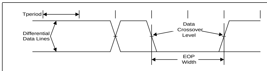
Figure 8-18. SMBus Transaction
