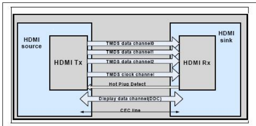
Figure 5-18. HDMI Overview
