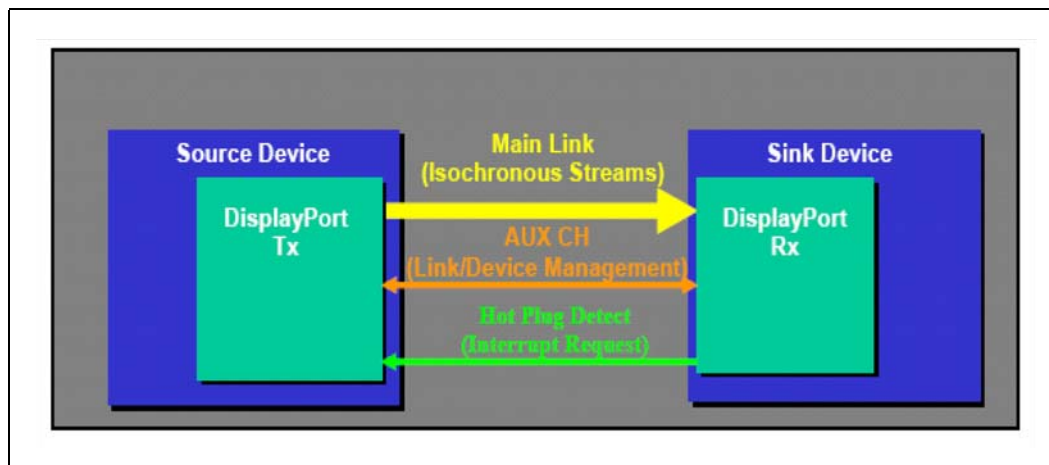
Figure 5-19. DP Overview
