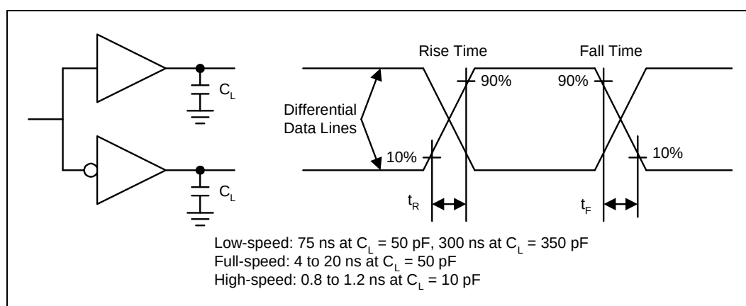
Figure 8-15. USB Rise and Fall Times
