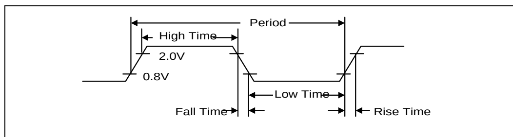
Figure 8-9. Clock Timing
