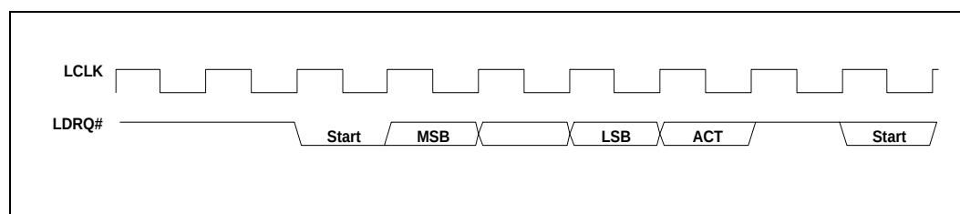
Figure 5-4. DMA Request Assertion through LDRQ#
