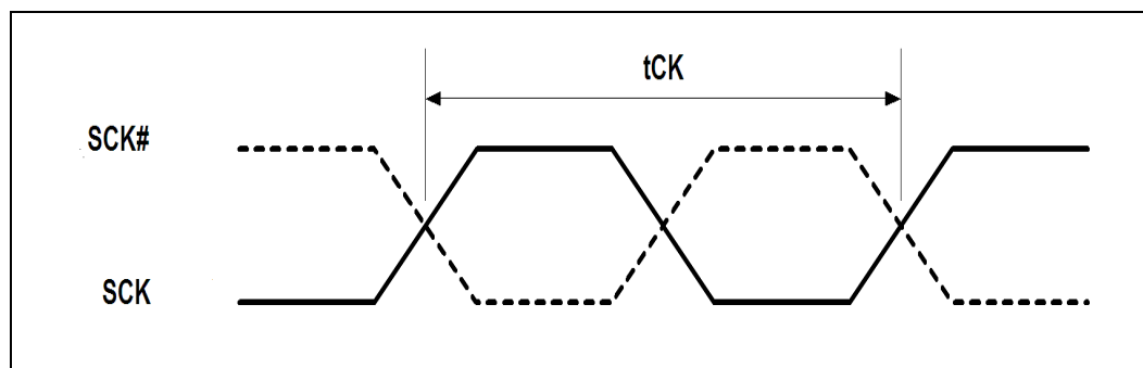
Figure 8-7. Clock Cycle Time
