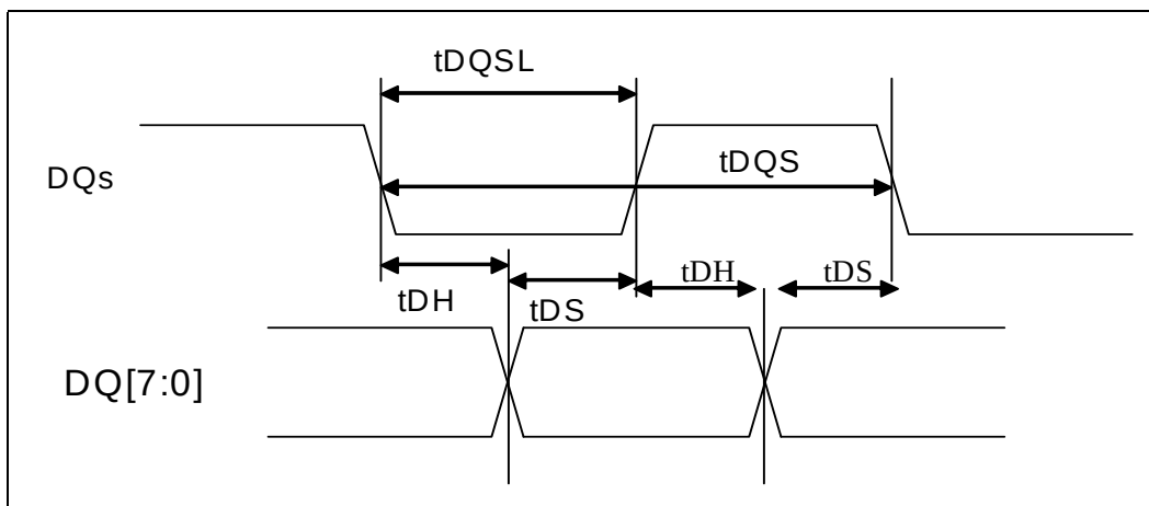
Figure 8-23. Dual Channel Interface Timings
