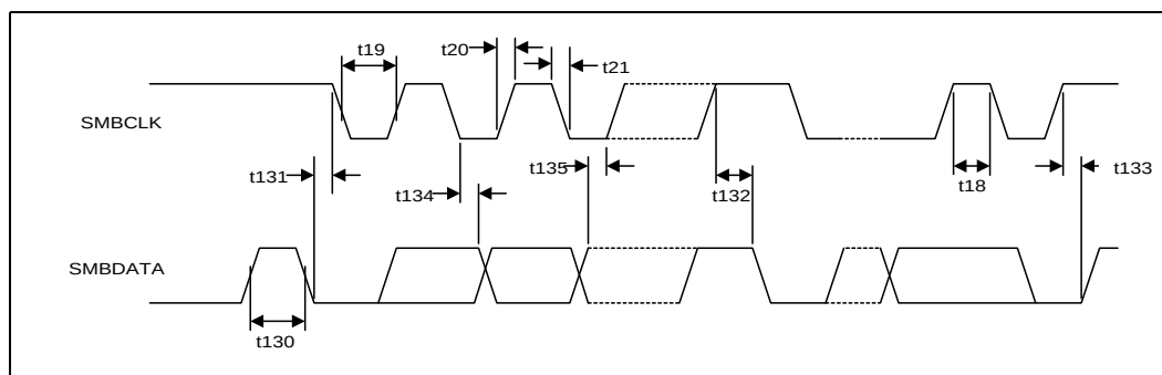
Figure 8-19. SMBus Timeout
