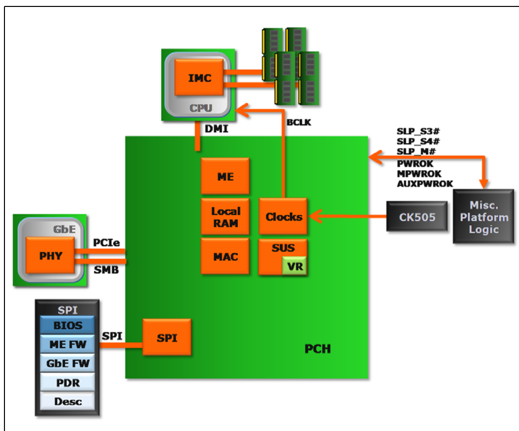
Figure 5-11. PCH Intel® Management Engine High-Level Block Diagram
