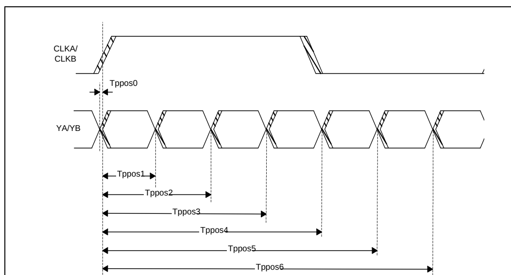
Figure 8-8. Transmitting Position (Data to Strobe)
