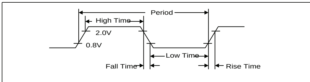
Figure 8-9. Clock Timing
