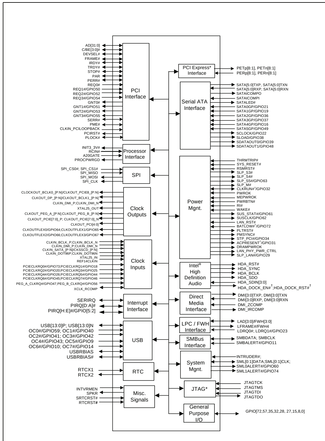
Figure 2-1. PCH Interface Signals Block Diagram
