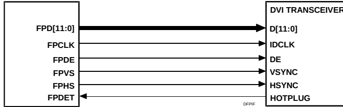
Figure 4. DVI Interface
