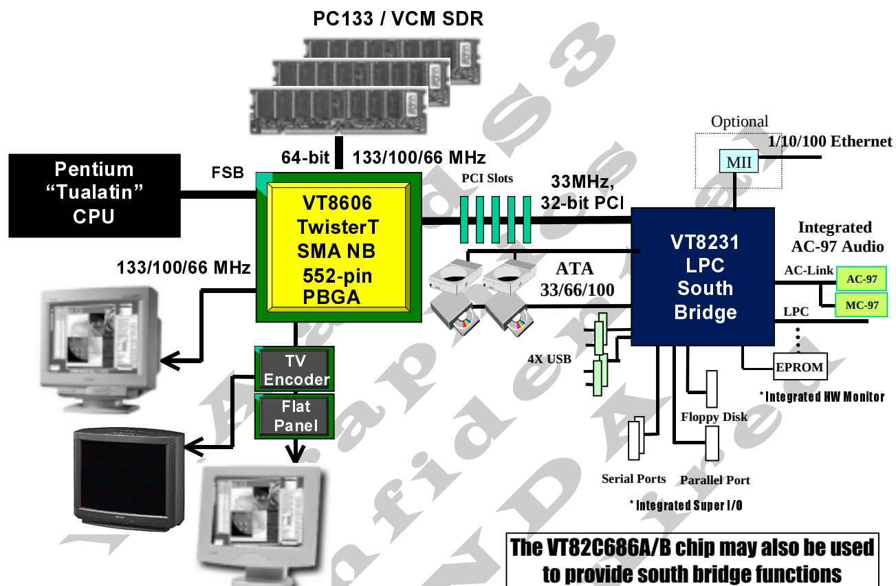
Figure 1. TwisterT System Block Diagram with VT8231 PCI-LPC South Bridge
