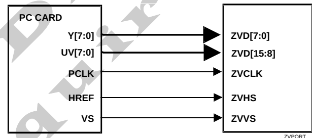
Figure 6. ZV-Port Interface
