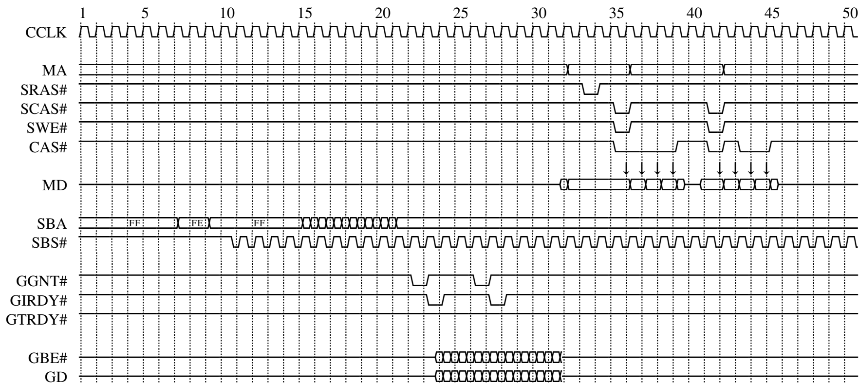
Figure 15. AGP Sideband Address 2x Write SDRAM
