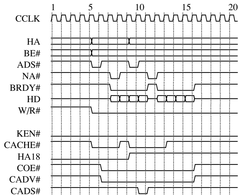
Figure 10. 2-Bank PBSRAM Read 3111-2111
