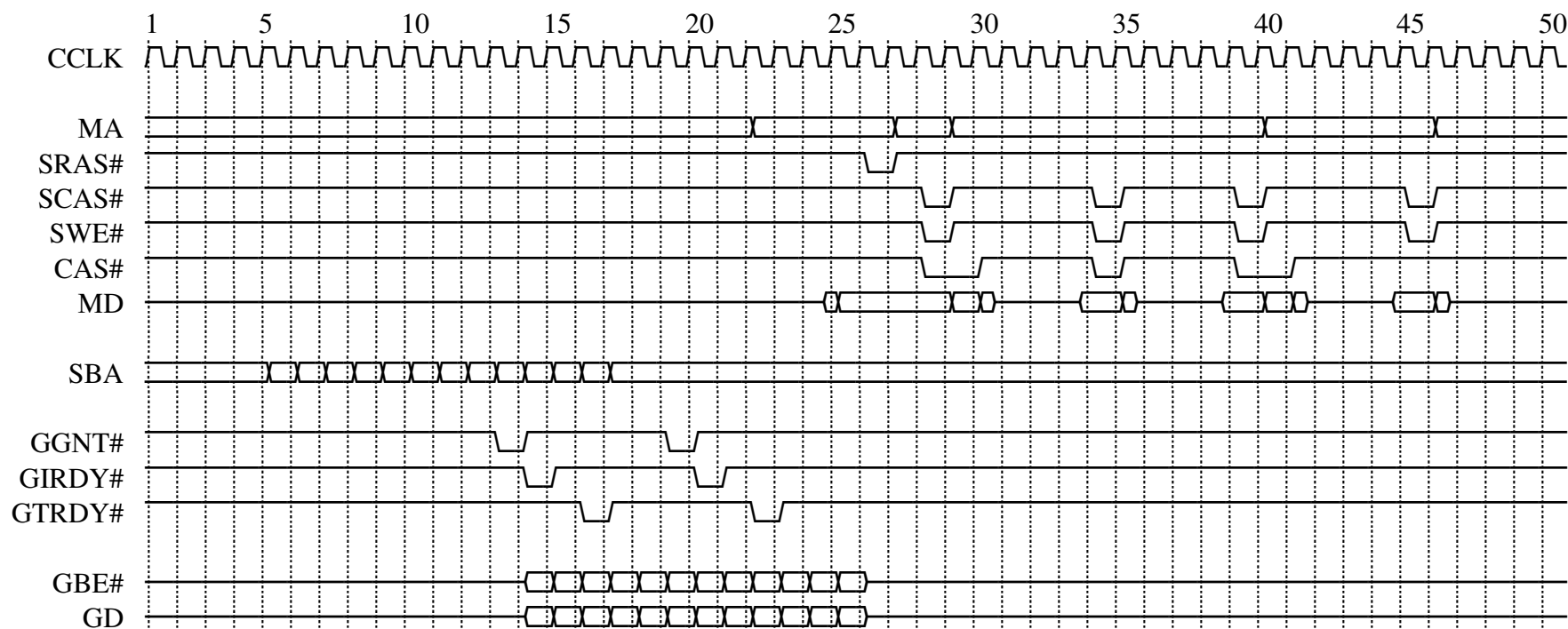
Figure 18. AGP Sideband Address 1x Write SDRAM
