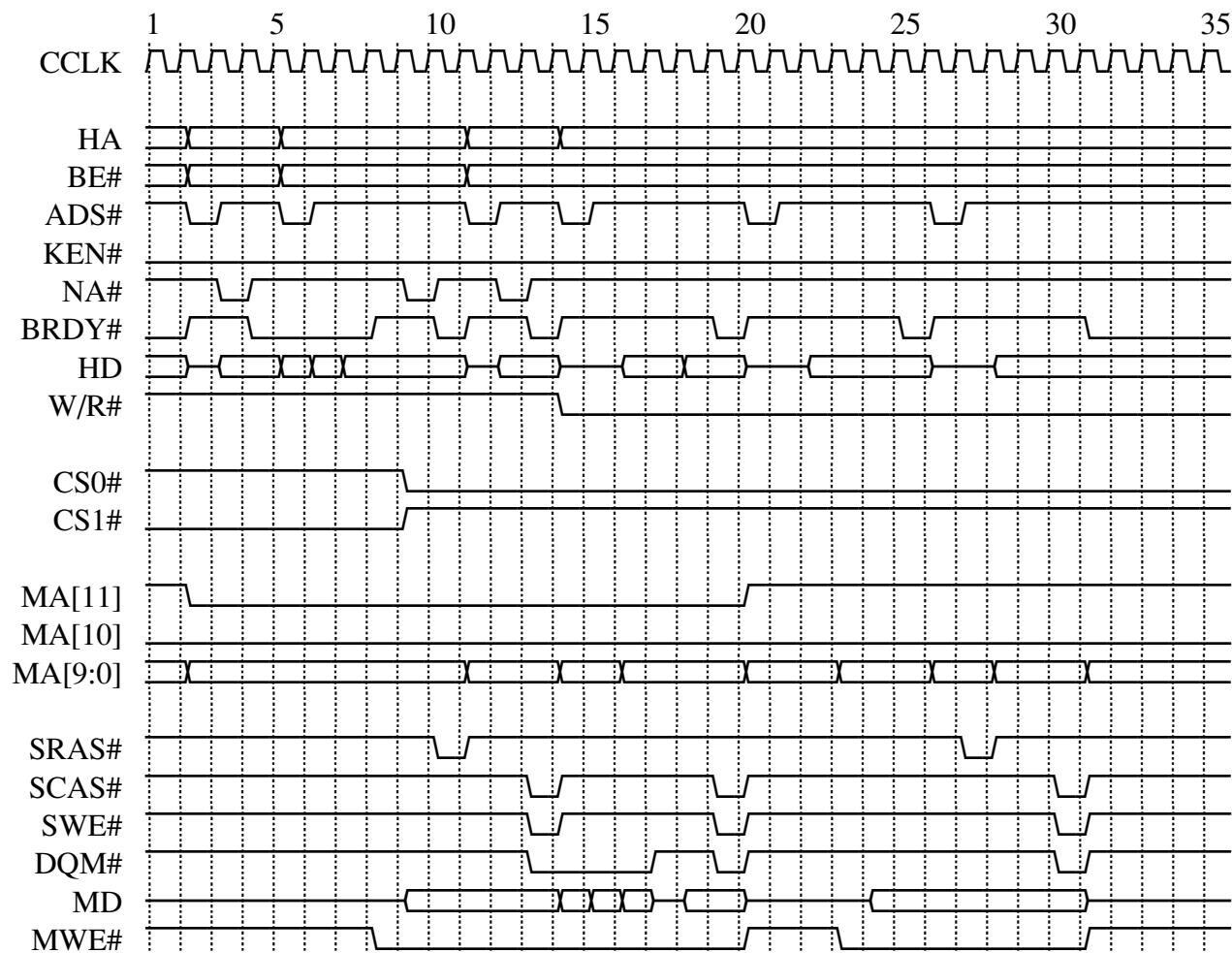
Figure 30. SDRAM Write Cycle (Bank Interleave)
