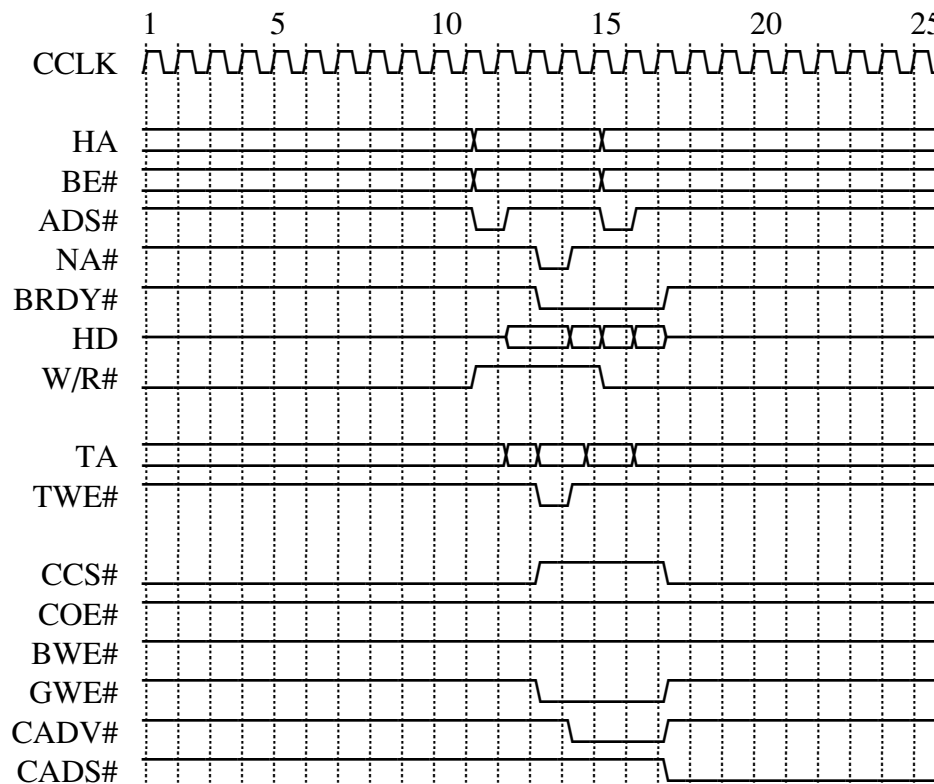
Figure 21. CPU Write Hit SRAM 3111
