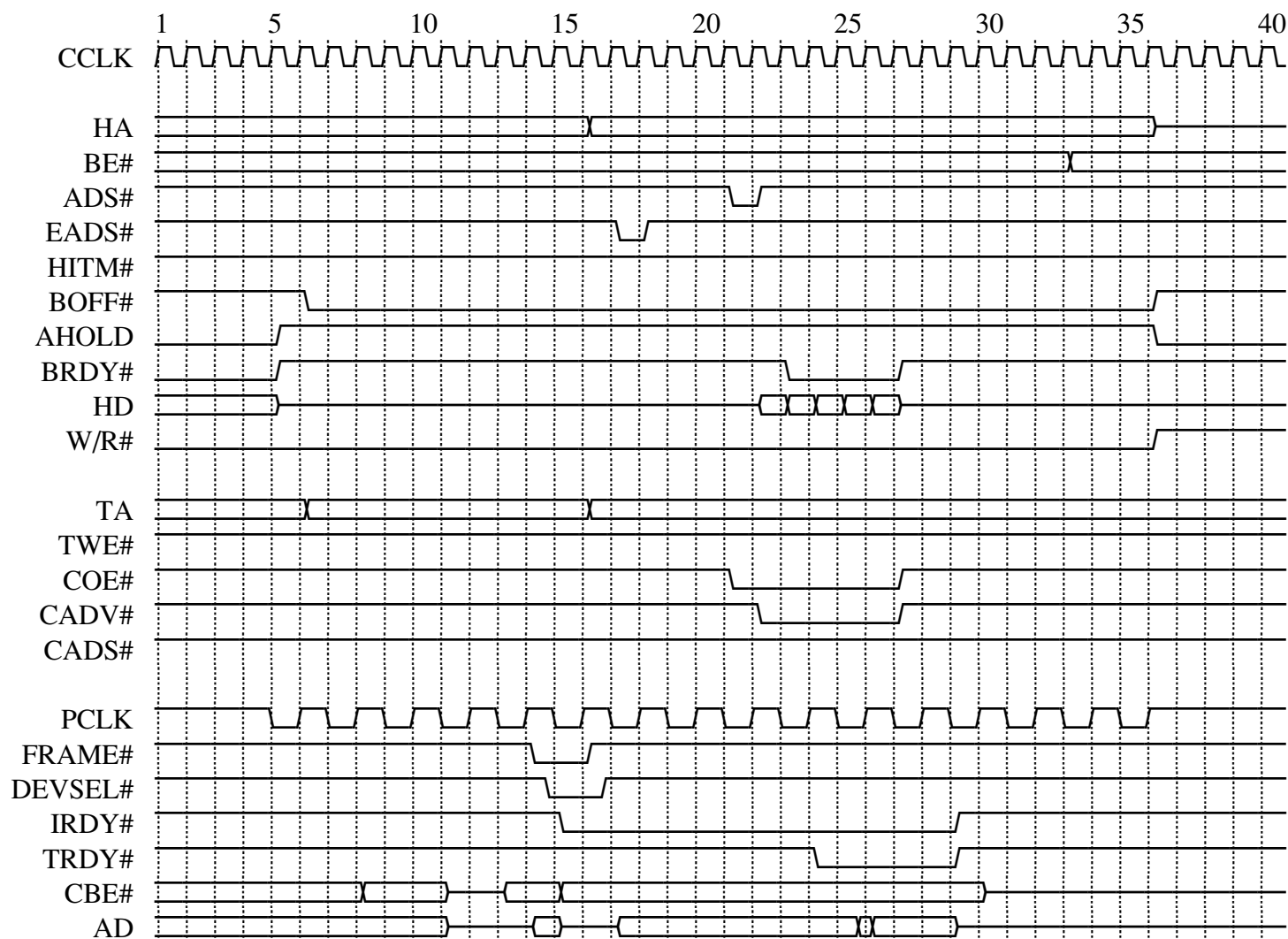
Figure 27. PCI Master Read Hit L2
