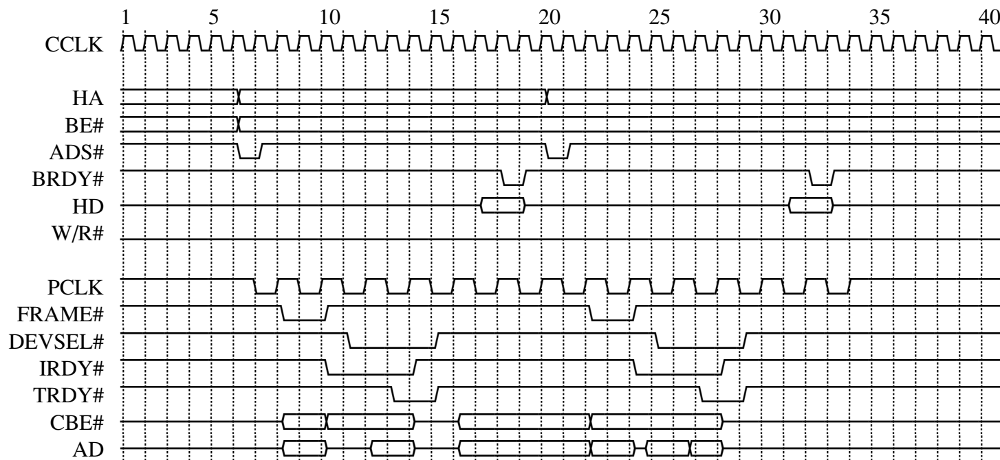
Figure 25. CPU Read PCI Slave
