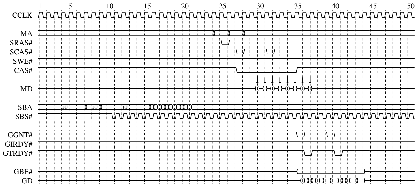
Figure 16. AGP Sideband Address 2x Read SDRAM (2L)
