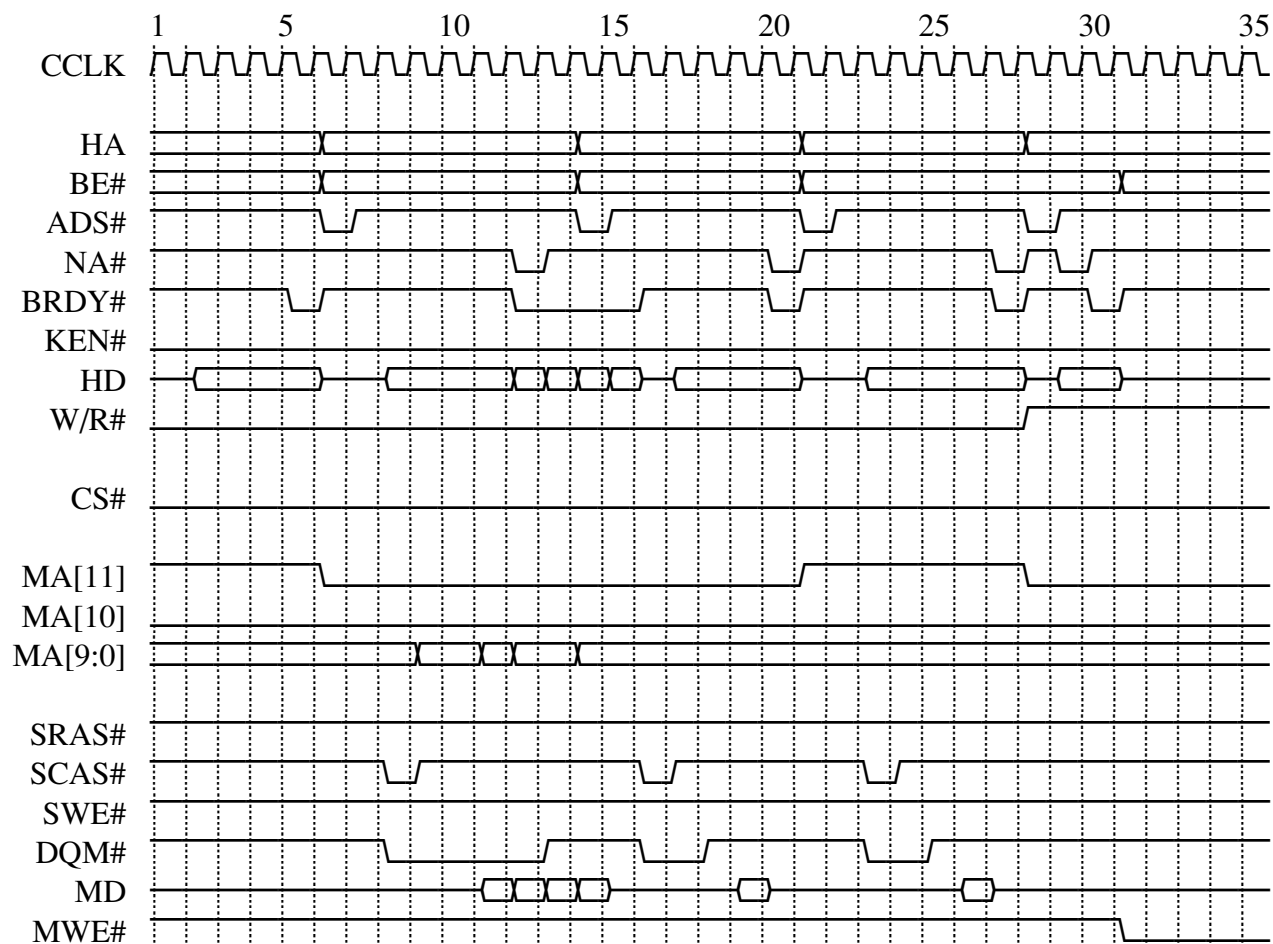
Figure 29. SDRAM Read Cycle (Bank Interleave, CAS Latency 3)
