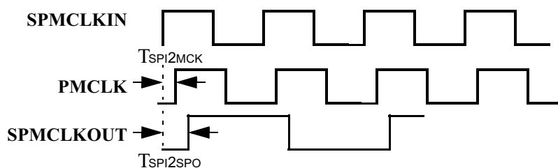
Figure 5-3. Master Clock Delay
