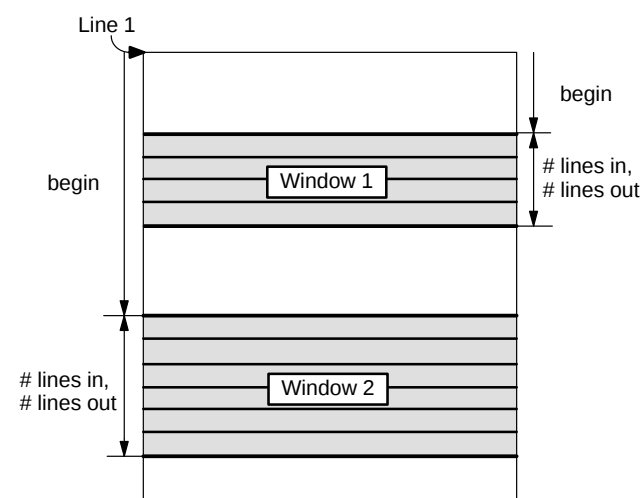
Fig. 2–31: Vertical dimensions of windows
