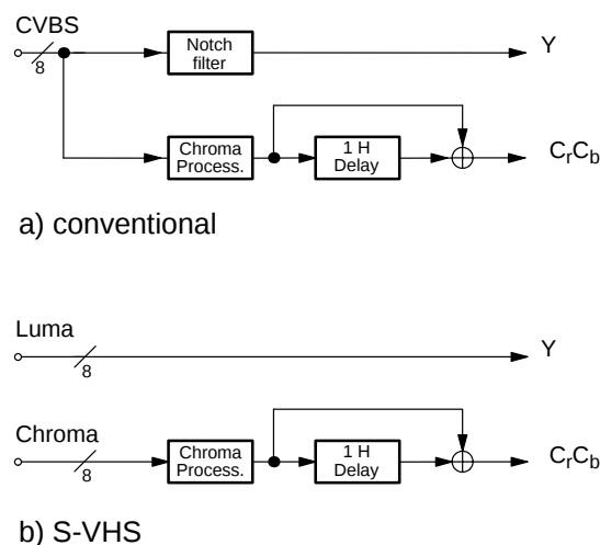
Fig. 2-8: PAL color decoding options
