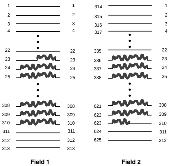
Fig. 2–34: Mapping for 625/50 line systems
