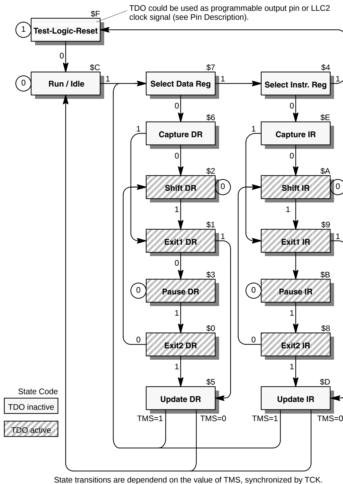
Fig. 2-42: TAP state transitions
