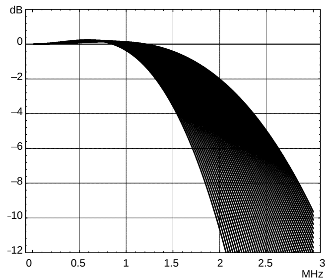
Fig. 2–13: Freq. response of 50 neighbored filters
