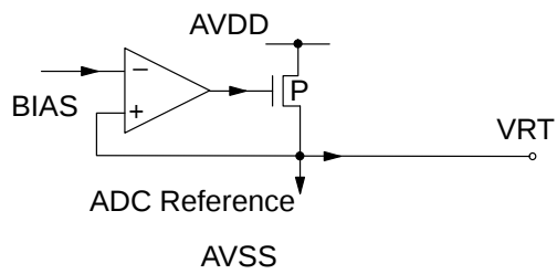
Fig. 3-9: Reference Voltage VRT
