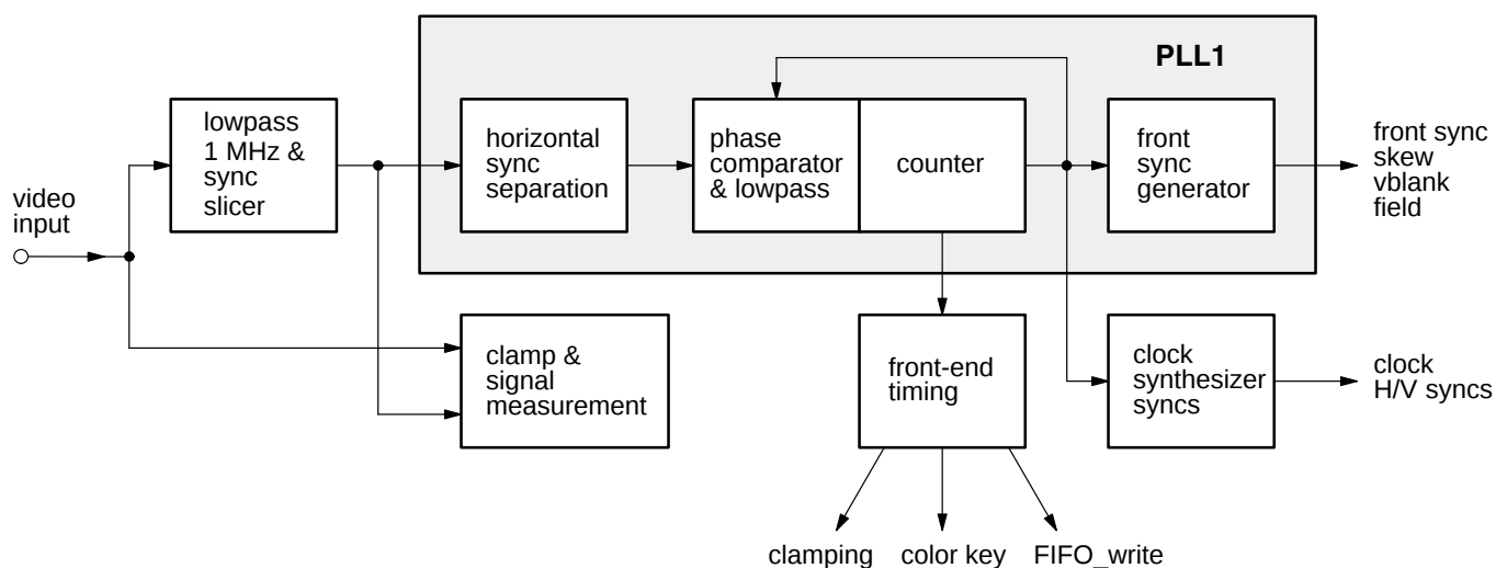
Fig. 2–10: Sync separation block diagram
