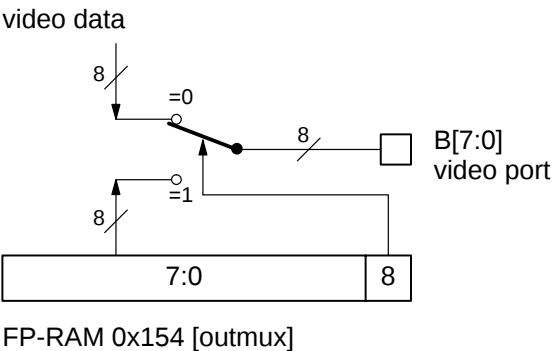
Fig. 2–21: Programmable output port
