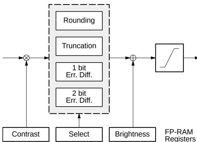
Fig. 2–15: Contrast and brightness adjustment
