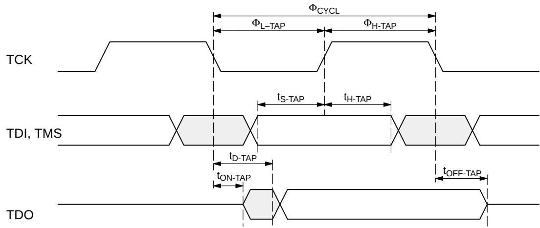
Fig. 5–5: Timing of Test Access Port TAP
