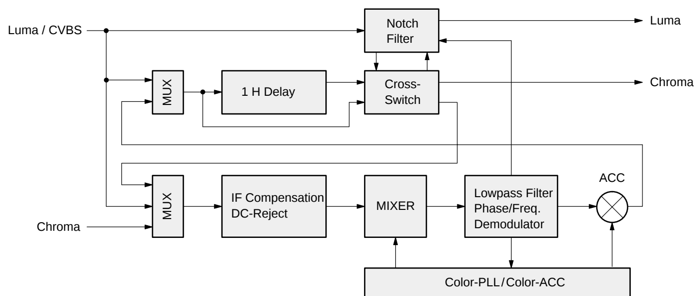
Fig. 2–4: Color decoder
