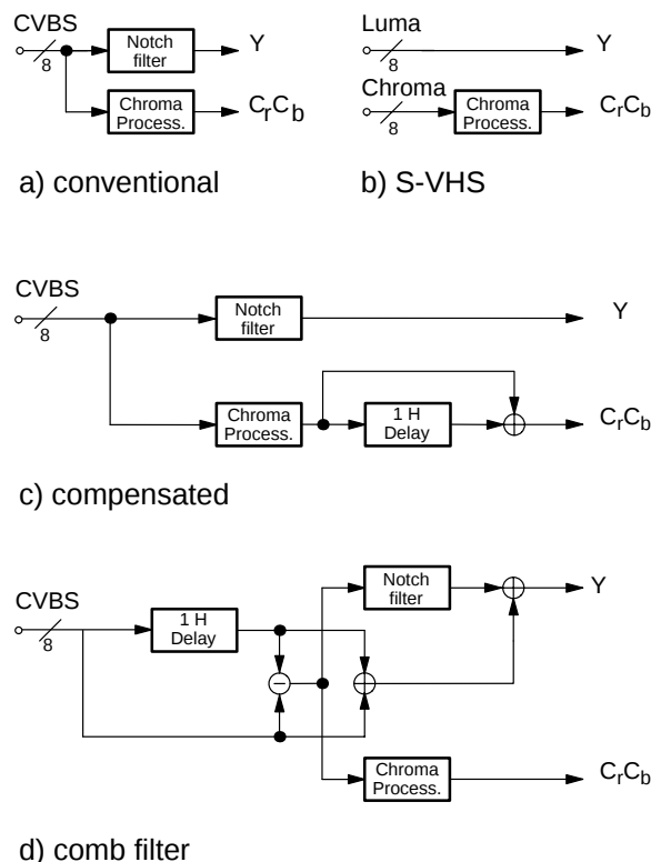
Fig. 2-7: NTSC color decoding options
