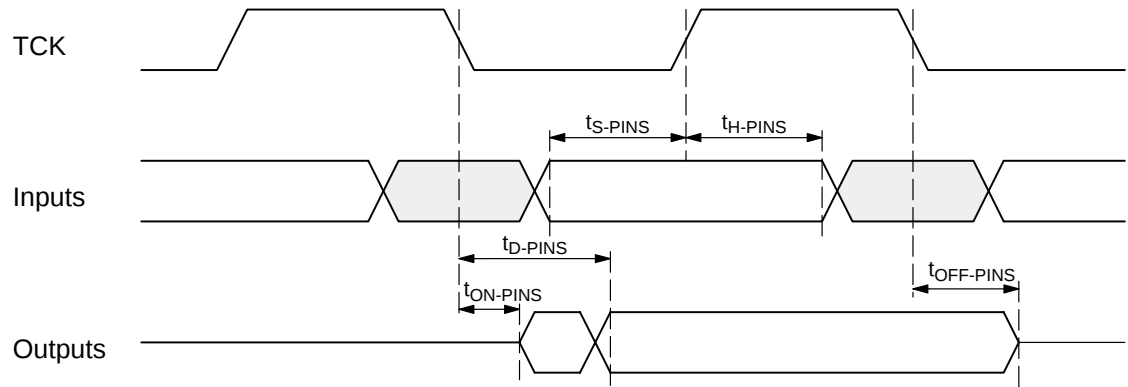
Fig. 5–6: Timing with respect to input and output signals
