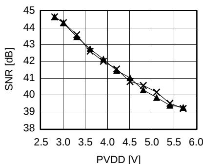
Fig. 7–1: Dependency between SNR and Power Supply
