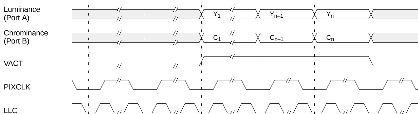
Fig. 2–17: Detailed data output (single clock mode)
