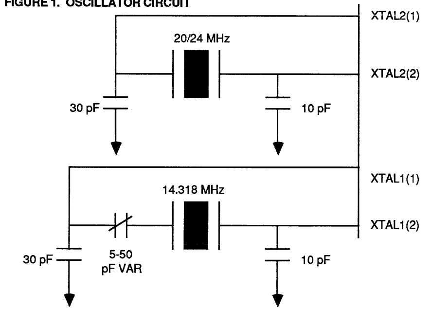
FIGURE 1. OSCILLATOR CIRCUIT
