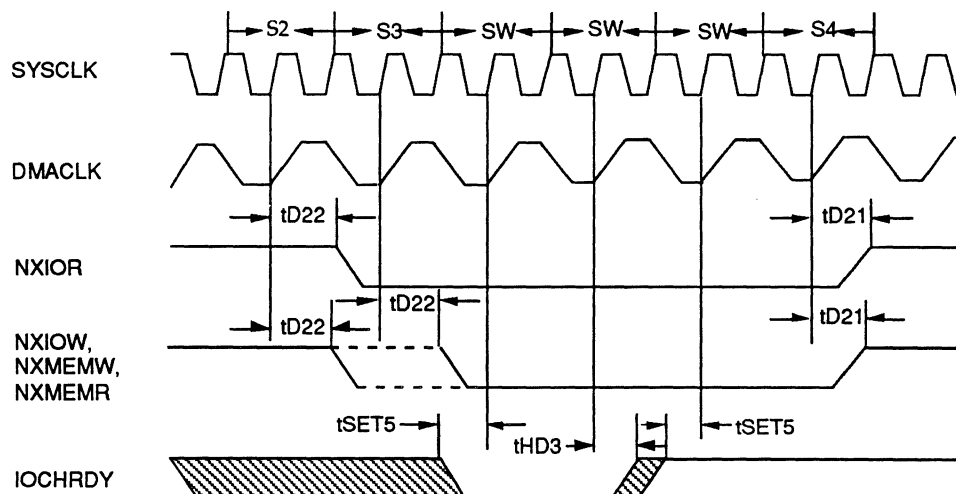
Figure 11. IOCHRDY TIMING
