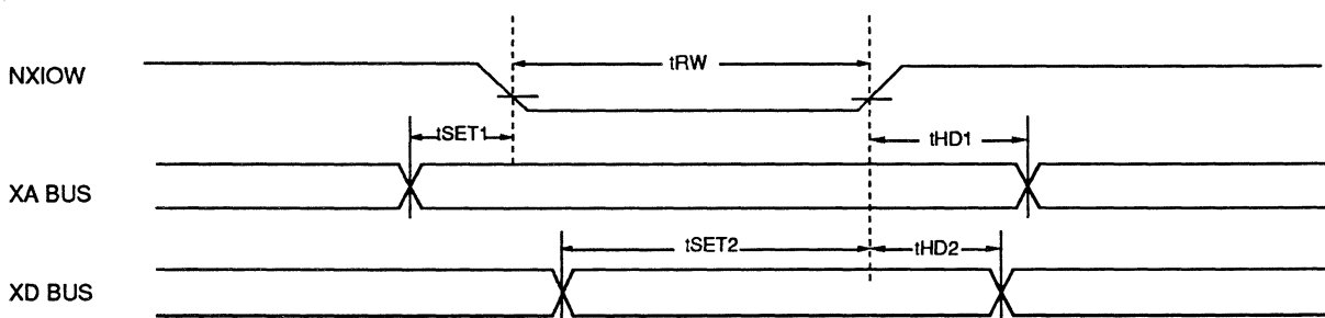
Fig. 5. WRITE TIMING
