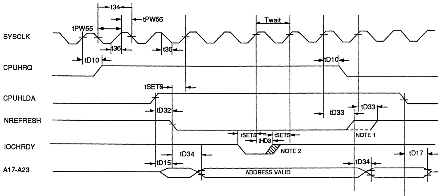
Figure 13. NREFRESH TIMING
