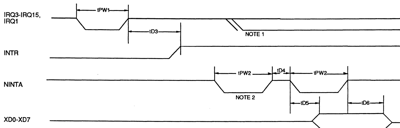
Fig. 7. INTERRUPT TIMING
