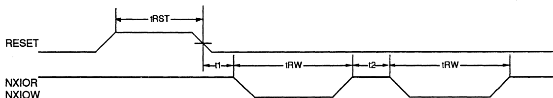
Fig. 6. COMMAND AND RESET TIMING
