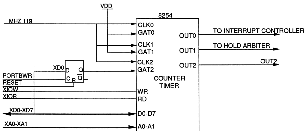
Fig. 3. Timer/Counter Subsection
