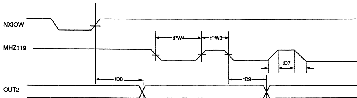
Fig. 8. TIMER/COUNTER TIMING
