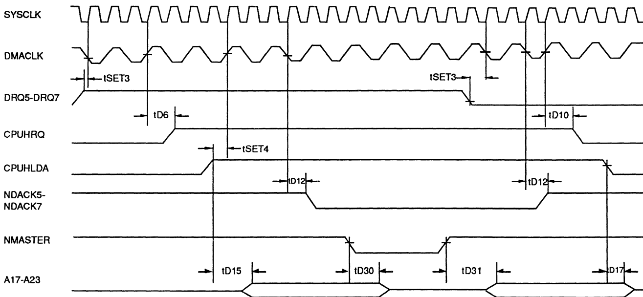
Figure 12. NMASTER TIMING
