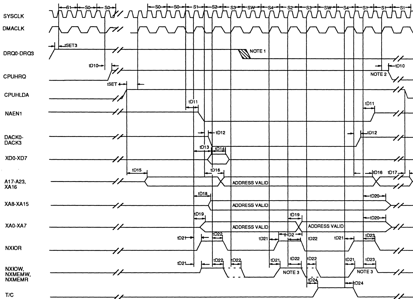
Figure 9. 8 BIT DMA TIMING
