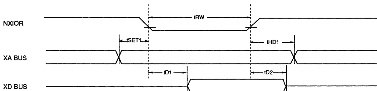
Fig. 4. READ TIMING
