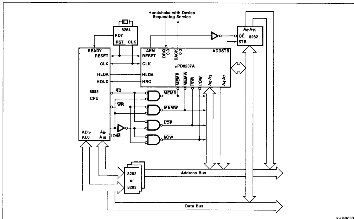
Figure 2. \mu PD8237A DMA Controller Application with 8088 CPU
