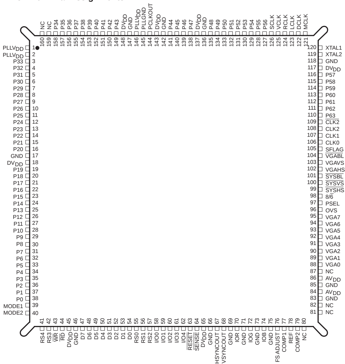
Figure 1–2. Terminal Assignments
