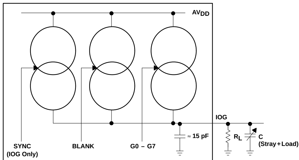
Figure 2–13. Equivalent Circuit of the Current Output (IOG)
