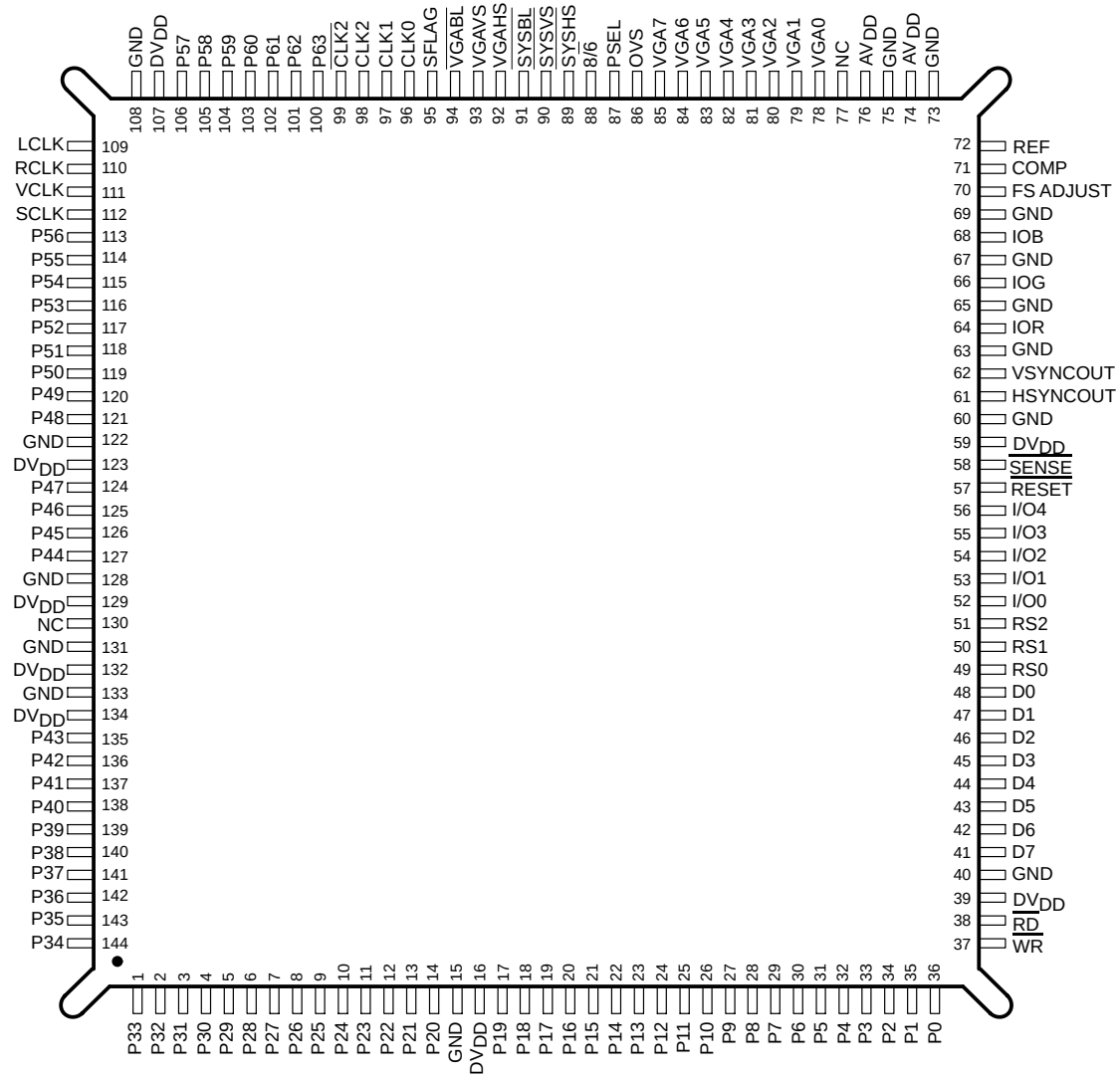
Figure 1–2. Terminal Assignments
