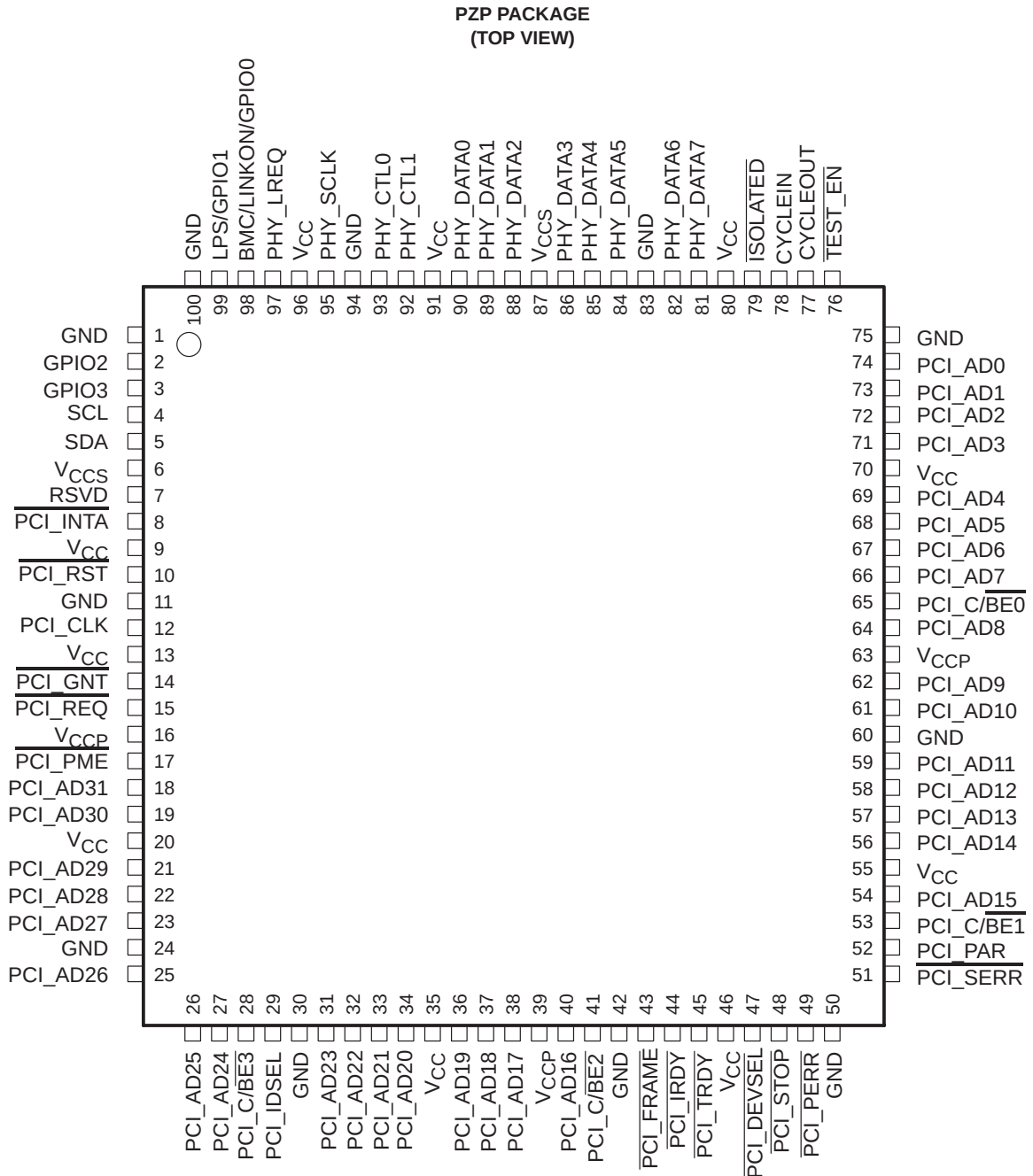
Figure 2. Terminal Assignments
