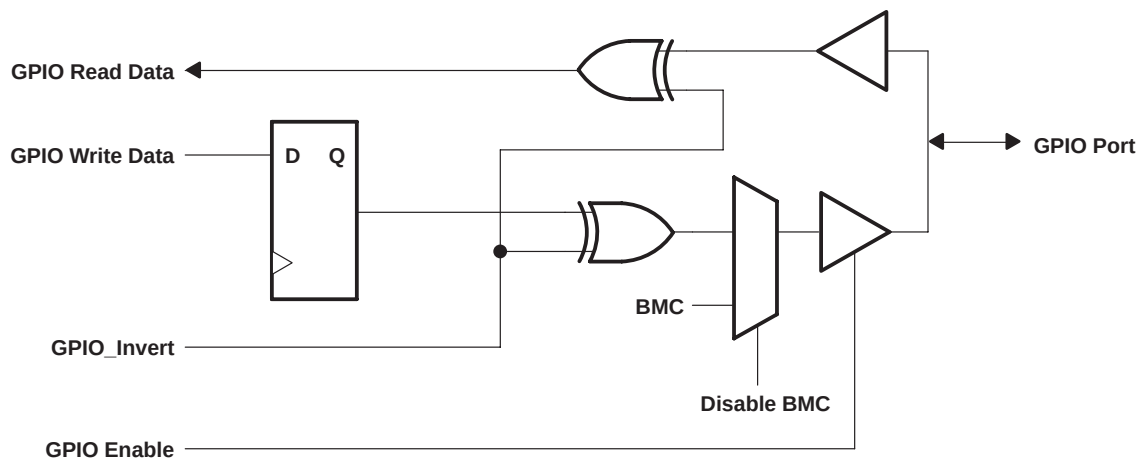
Figure 3. BMC/LINKON/GPIO0
