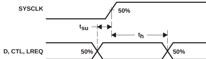
Figure 1. D, CTL, LREQ Input Setup and Hold Timing Waveforms
