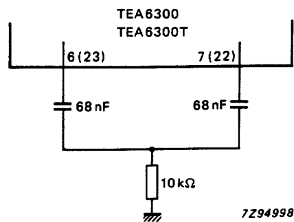
Fig.5 T-pass filter.
