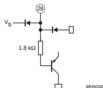
Fig.25 Pin 28; MAD.
