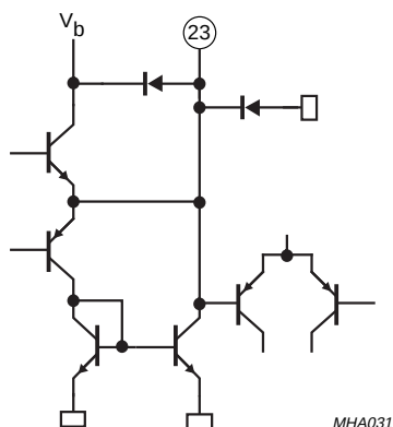
Fig.22 Pin 23; SAP.
