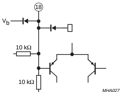
Fig.18 Pin 18; C MO and pin 19; C SS .
