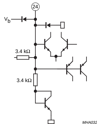
Fig.23 Pin 24; V ref .
