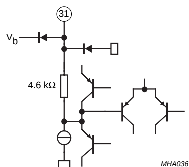
Fig.27 Pin 31; C W and pin 32; C S .
