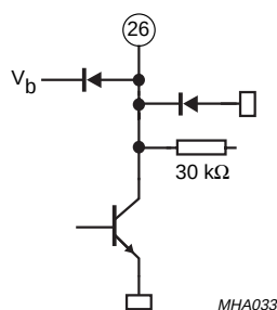
Fig.24 Pin 26; C ND .
