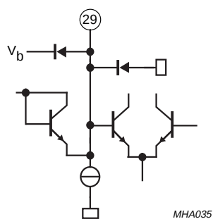
Fig.26 Pin 29; C TW and pin 30; C TS .
