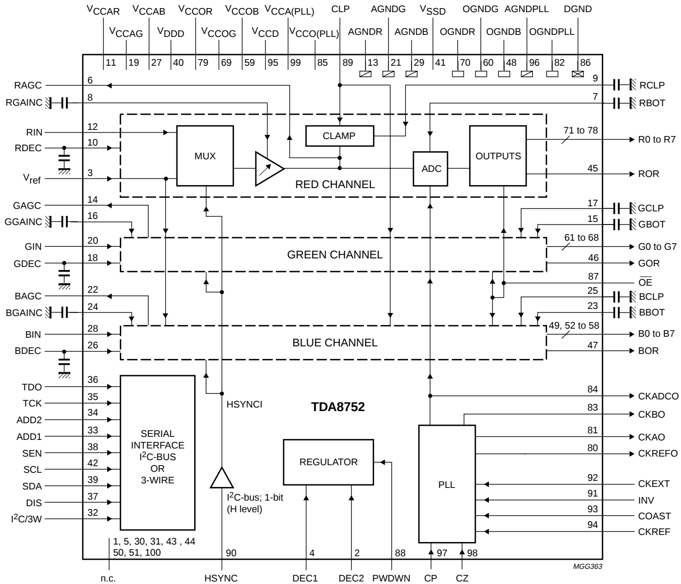
Fig.1 Block diagram.
