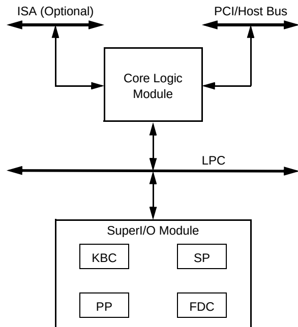
Figure 5-15. Typical Setup
