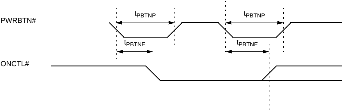
Figure 7-47. PWRBTN# Trigger and ONCTL# Timing
