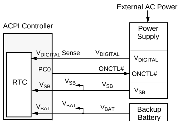
Figure 4-8. Power Supply Connections
