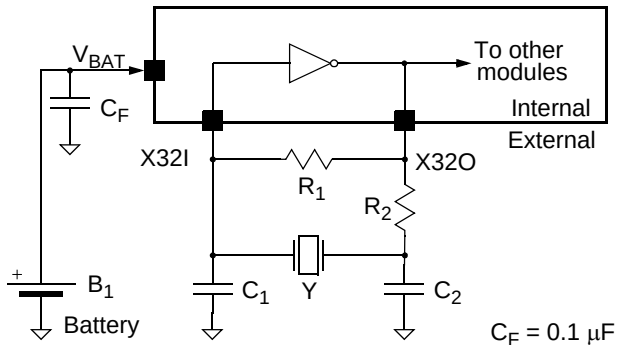
Figure 4-5. Recommended Crystal External Circuitry
