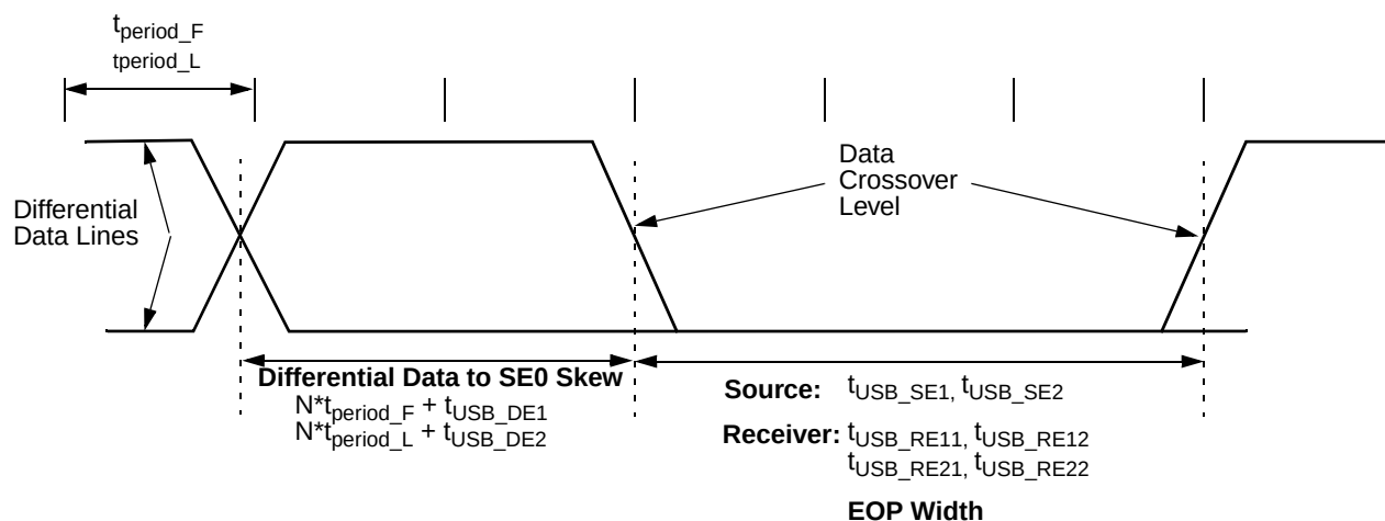
Figure 7-37. EOP Width Timing
