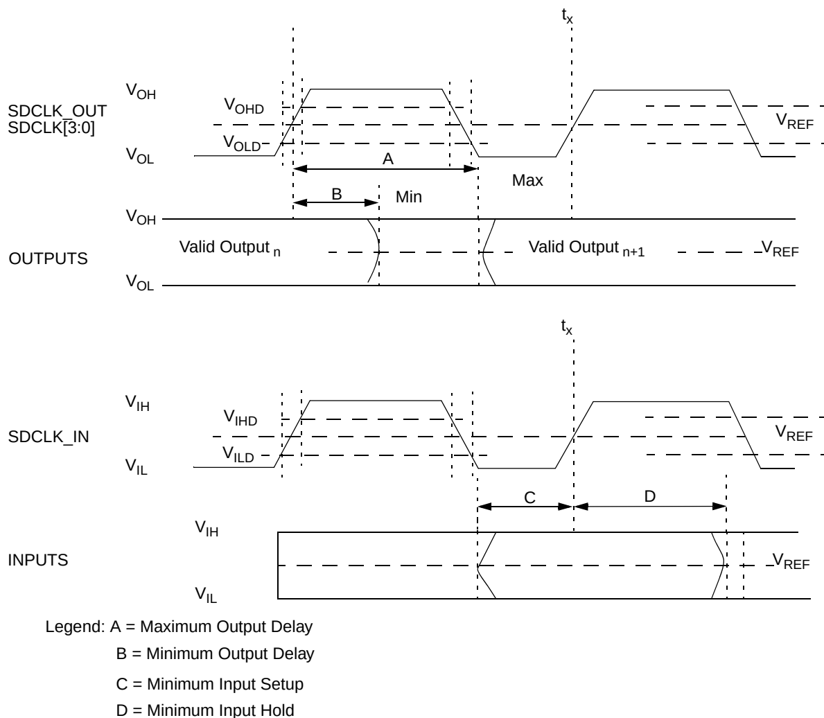
Figure 7-3. Drive Level and Measurement Points for Switching Characters
