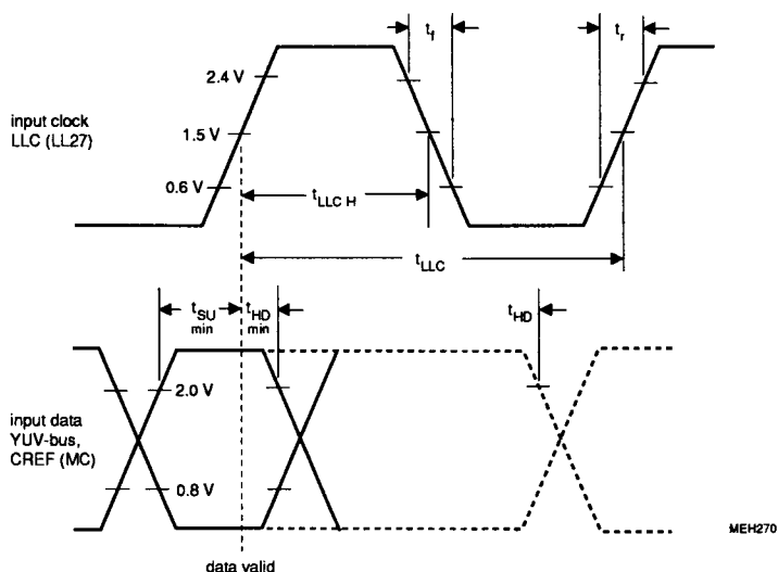
Fig.4 YUV-bus data and CREF timing.
