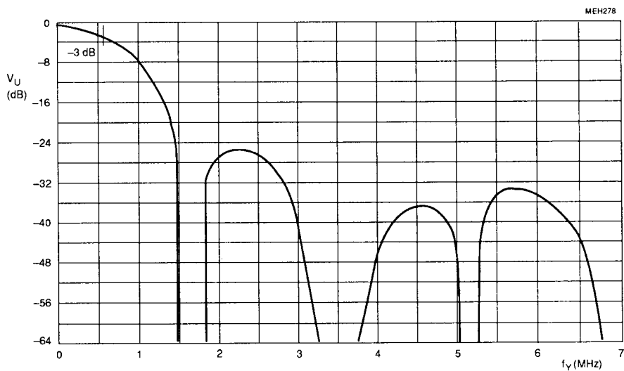
Fig.11 Interpolation filter with I 2 C-bus control bits IFF = 0; IFC = 0 and IFL = 1 in 4:1:1 format, and control bits IFF = 1; IFC = 0 and IFL = 1 in 4:2:2 format; 13.5 MHz data rate.
