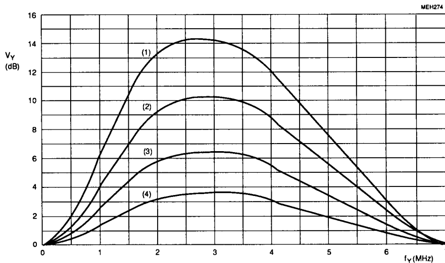
Fig. 8 Peaking frequency response with I 2 C-bus control bits BP1 = 1; BP0 = 1 and BFB = 0: (1) K = 1 ; (2) K = 1/2 ; (3) K = 1/4 and (4) K = 1/8 .
