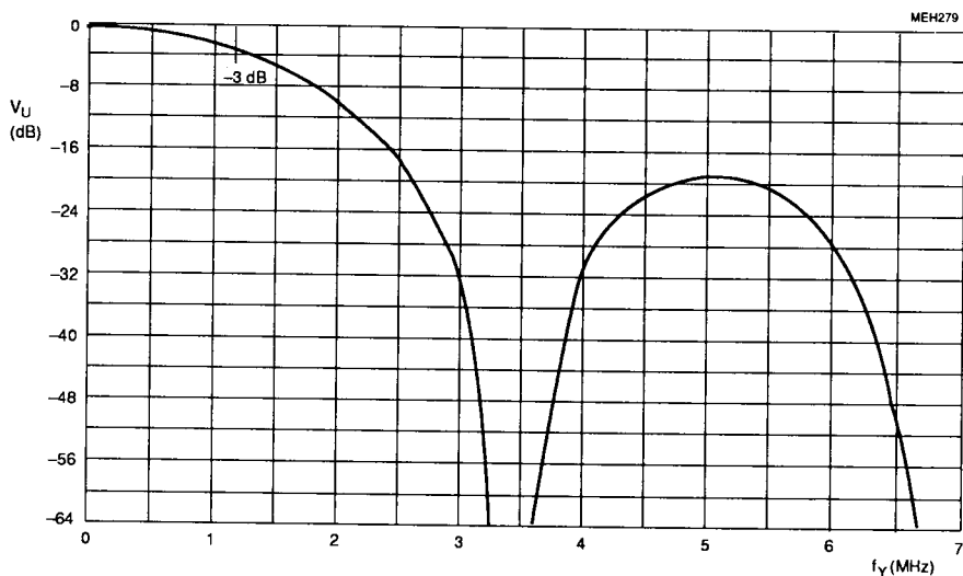
Fig.12 Interpolation filter with I 2 C-bus control bits IFF = 0; IFC = 1 and IFL = 0 in 4:1:1 format; 13.5 MHz data rate.
