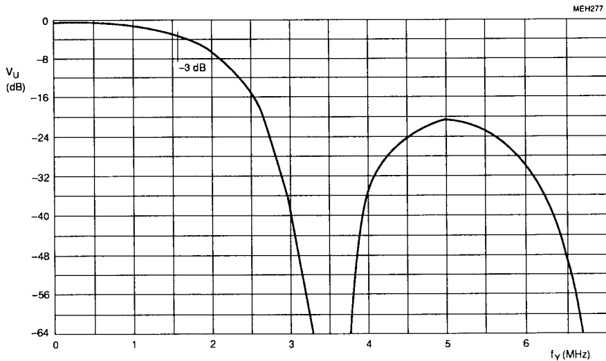
Fig.10 Interpolation filter with I 2 C-bus control bits IFF = 0; IFC = 0 and IFL = 0 in 4:1:1 format, and control bits IFF = 1; IFC = 0 and IFL = 0 in 4:2:2 format; 13.5 MHz data rate.
