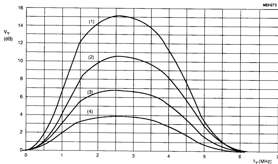
Fig.6 Peaking frequency response with I 2 C-bus control bits BP1 = 0; BP0 = 1 and BFB = 0: (1) K = 1 ; (2) K = 1/2 ; (3) K = 1/4 and (4) K = 1/8 .
