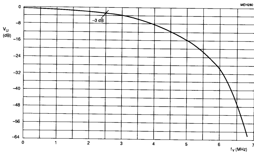
Fig.13 Interpolation filter with I 2 C-bus control bits IFF = 1; IFC = 1 and IFL = X in 4:2:2 format; 13.5 MHz data rate.
