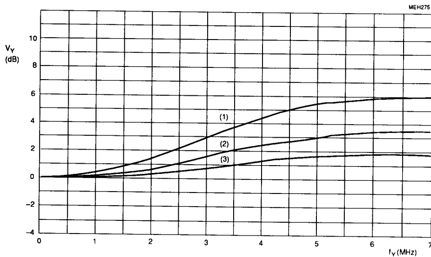
Fig.9 Peaking frequency response with I 2 C-bus control bits BP1 = 0; BP0 = 0 and BFB = 1; bandpass filter BF1 bypassed and peaking off; (1) K = 1 ; (2) K = 1/2 ; (3) K = 1/4 .
