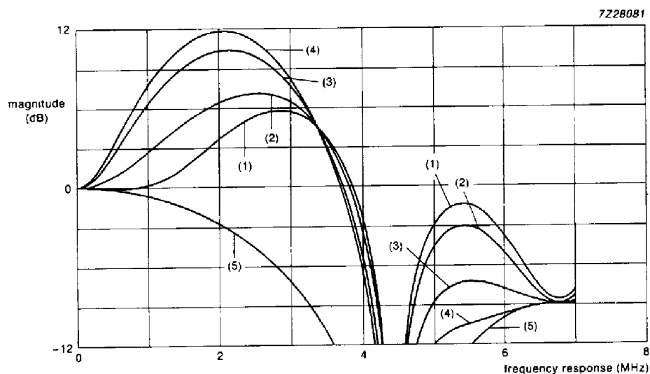
Fig.13 Magnitude of the frequency response of the unlimited summation signal (combining Channel 1 and Channel 2); PAL mode; prefilter OFF; Responses 1 to 5 show various comb-filter combinations programmable by bits BP2 and BP1, via the I 2 C-bus.
