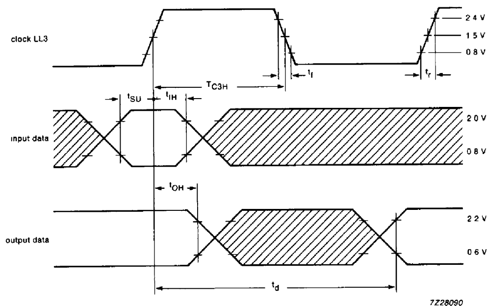
Fig.23 Timing diagram.
