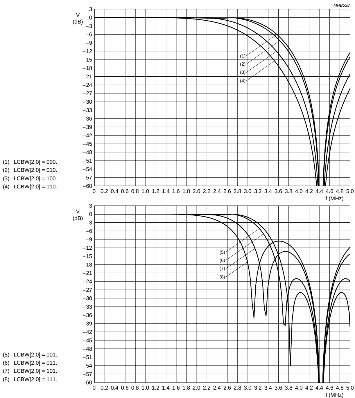
Fig.17 Transfer characteristics of the luminance notch filter in 4.43 MHz mode (Y-comb filter disabled) at LUBW = 1.
