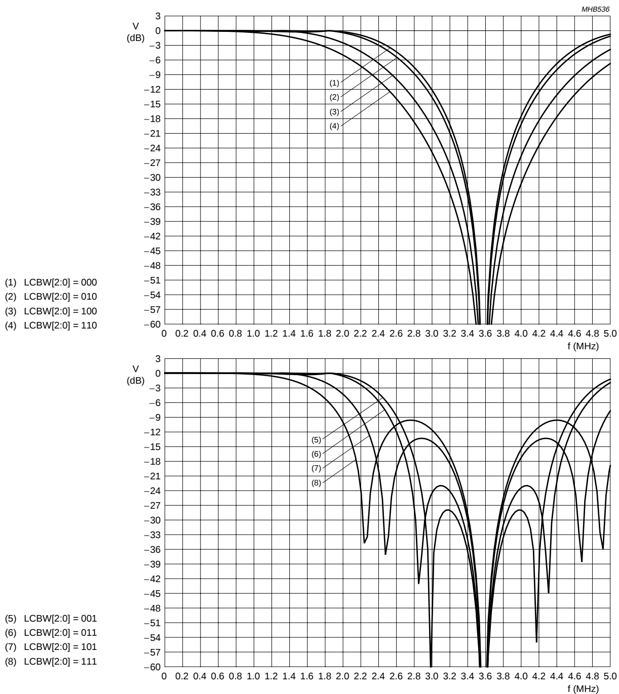
Fig.15 Transfer characteristics of the luminance notch filter in 3.58 MHz mode (Y-comb filter disabled) at LUBW = 1.
