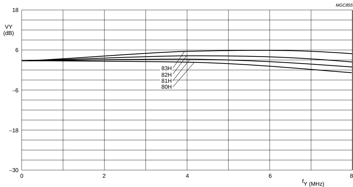
Fig.36 Luminance control: SU06H, 50 Hz/Y + C mode, prefilter off and coring off.
