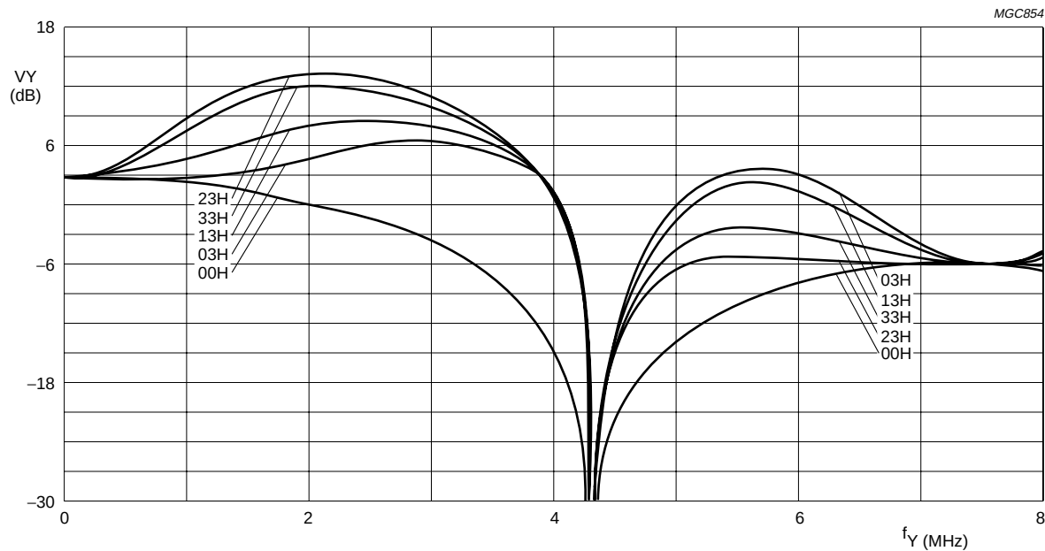
Fig.35 Luminance control: SU06H, 50 Hz/CVBS mode, prefilter off and coring off.
