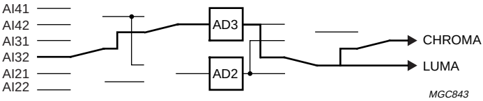
Fig.24 Mode 3; CVBS4.
