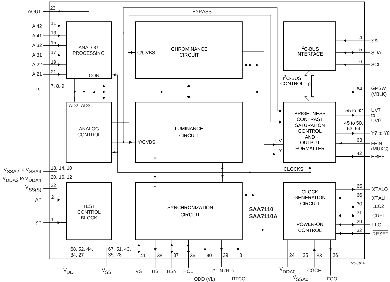
Fig.2 Block diagram.
