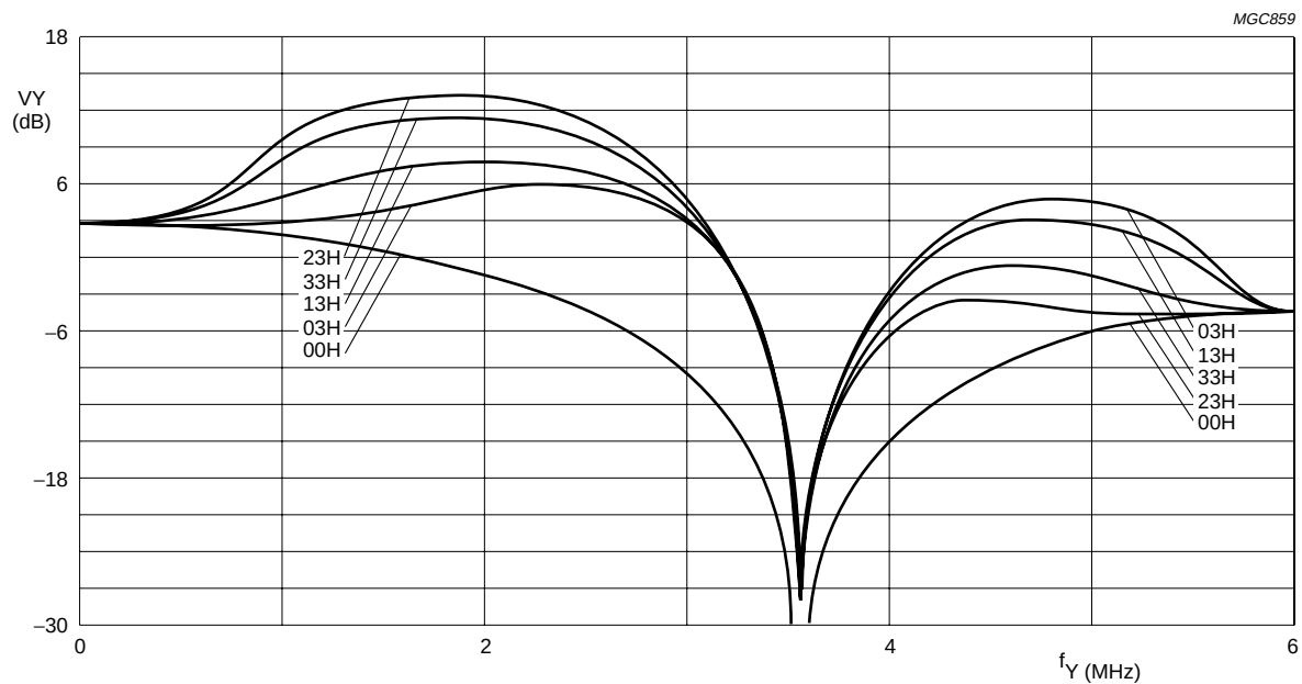
Fig.40 Luminance control: SU06H, 60 Hz/CVBS mode, prefilter off and coring off.
