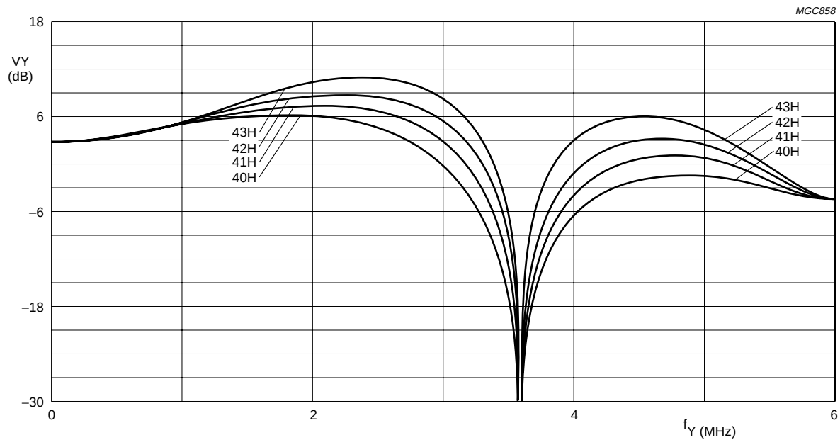
Fig.39 Luminance control: SU06H, 60 Hz/CVBS mode, prefilter on and coring off.
