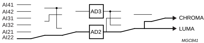
Fig.22 Mode 1; CVBS2.
