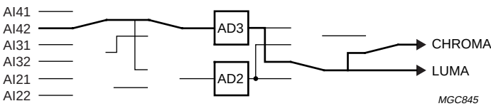
Fig.26 Mode 5; CVBS6.
