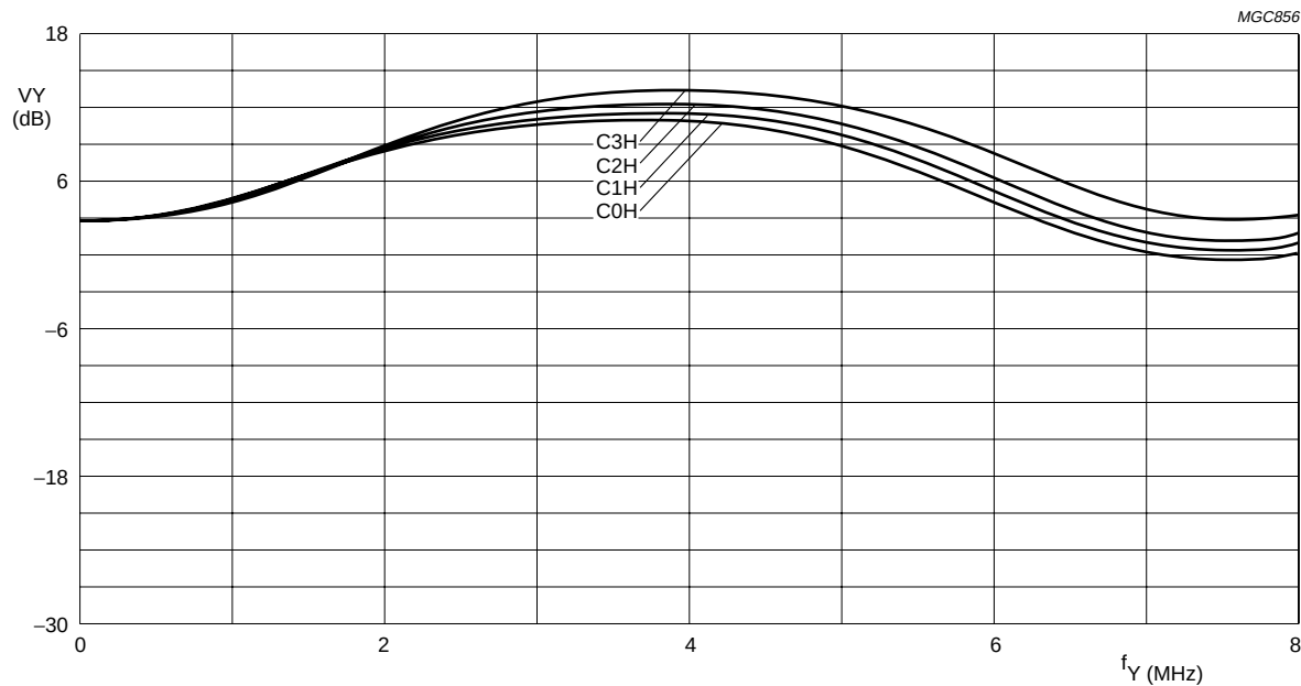
Fig.37 Luminance control: SU06H, 50 Hz/Y + C mode, prefilter on and coring off.
