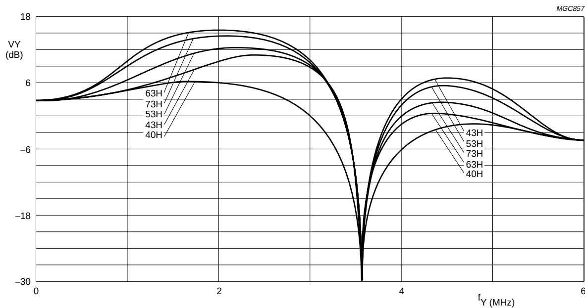
Fig.38 Luminance control: SU06H, 60 Hz/CVBS mode, prefilter on and coring off.
