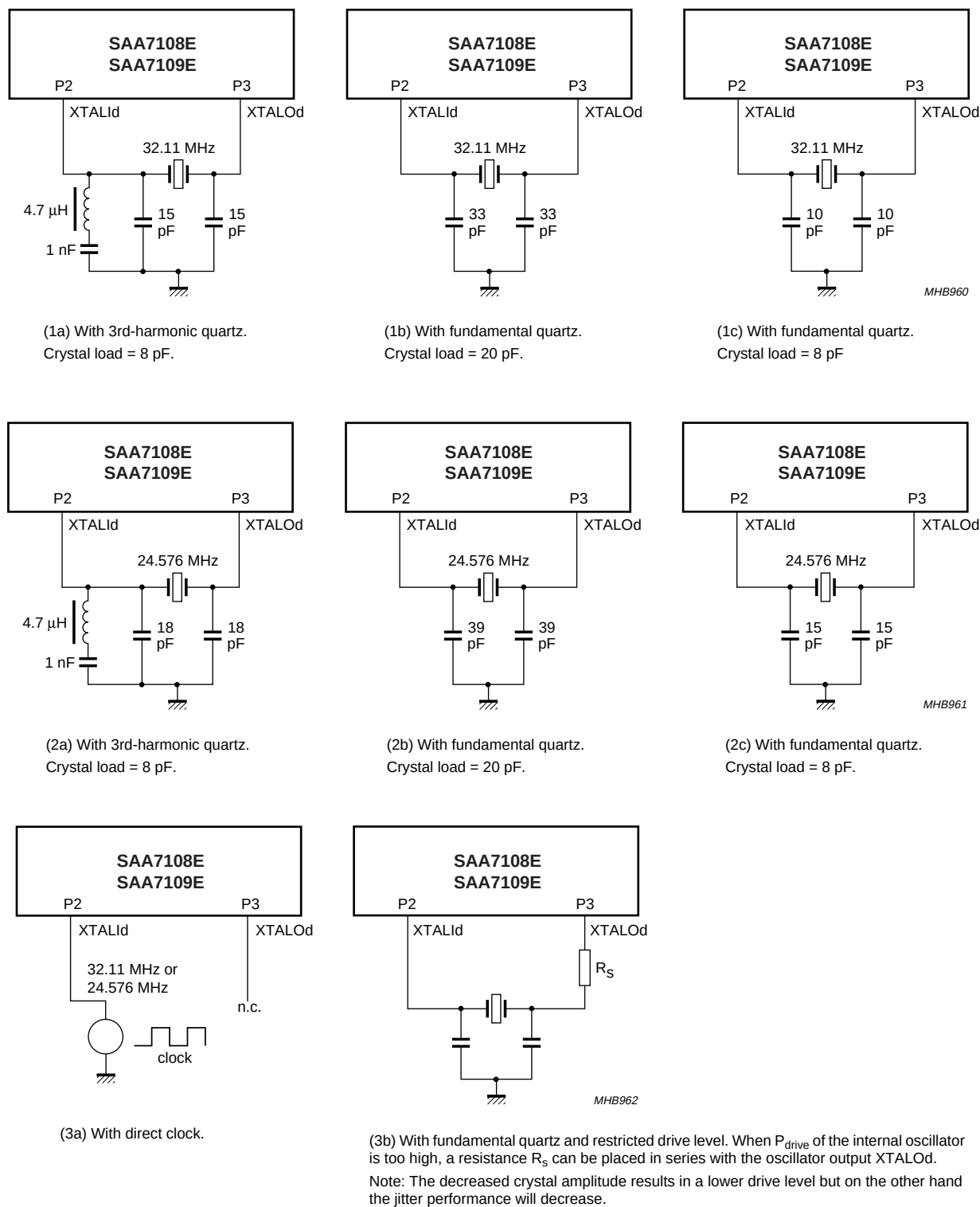
Fig.54 Oscillator application for decoder part.
