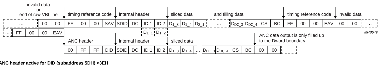
Fig.38 Sliced data formats on the I port in 8-bit mode.
