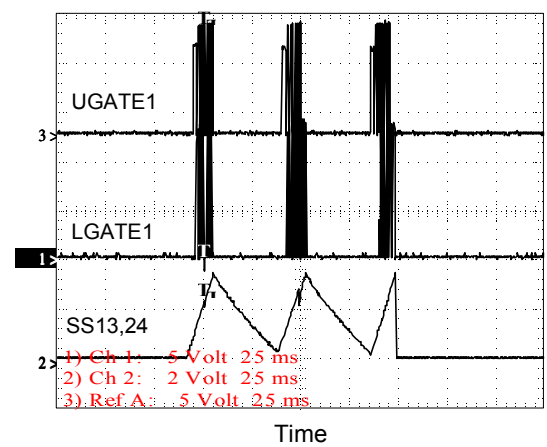
V_{OUT1} Short
