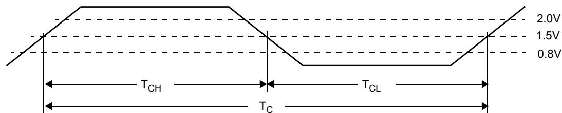
Figure 5. Timing Waveform
