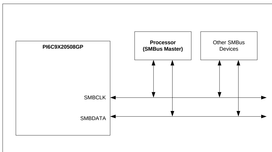
Figure 6-1 SMBus Architecture Implementation on PI7C9X20508GP
